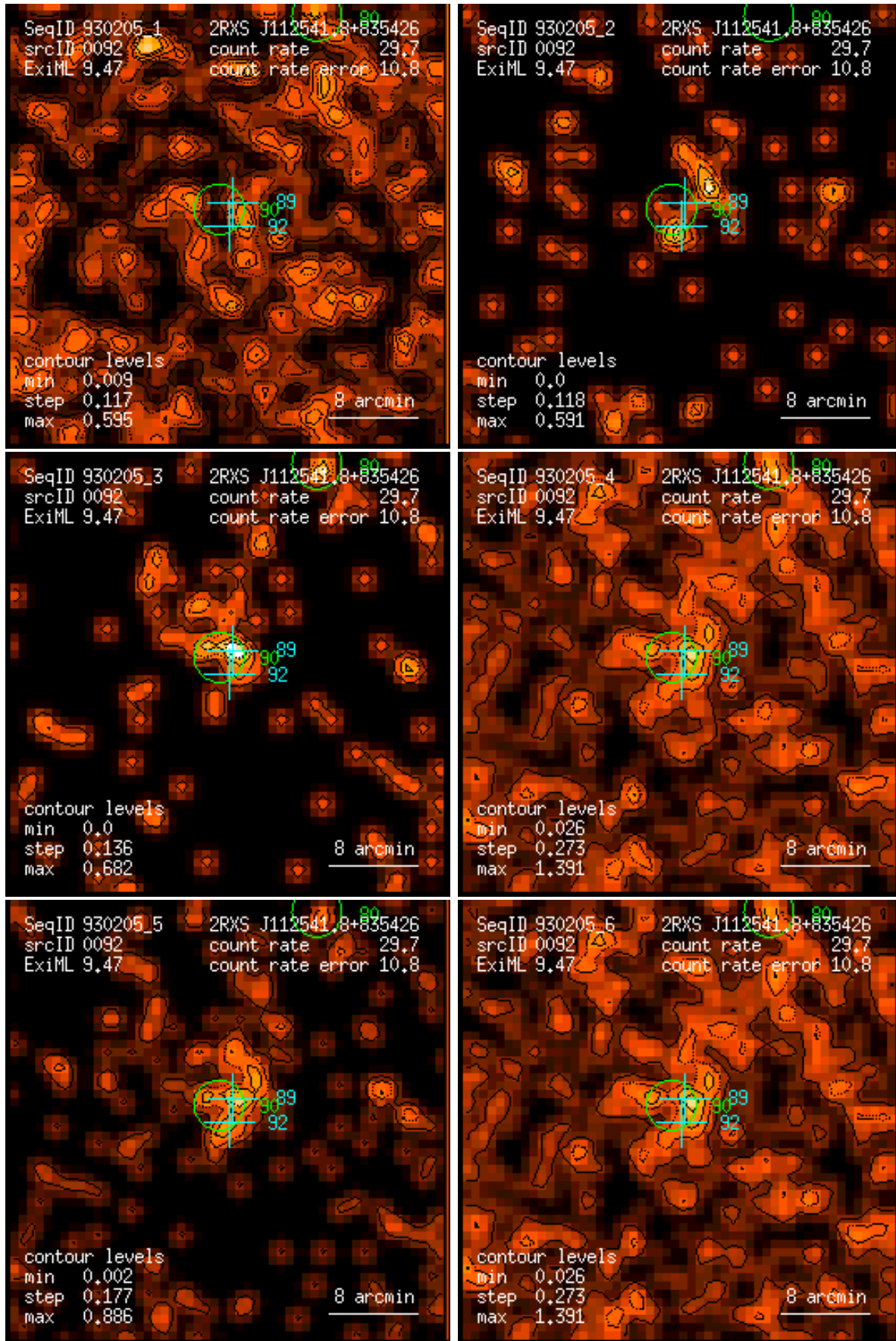
Figure 92: RASS 930205: detection 0092: band rate images, Gaussian filter: (1) PSPC channels 11 – 41, (2) 52 – 90, (3) 91 – 201, (4) 11 – 235, (5) 52 – 201, (6) 11 – 201. Broad band rates in counts/ks. Band rate contour levels in counts/ks/arcmin 2 .
