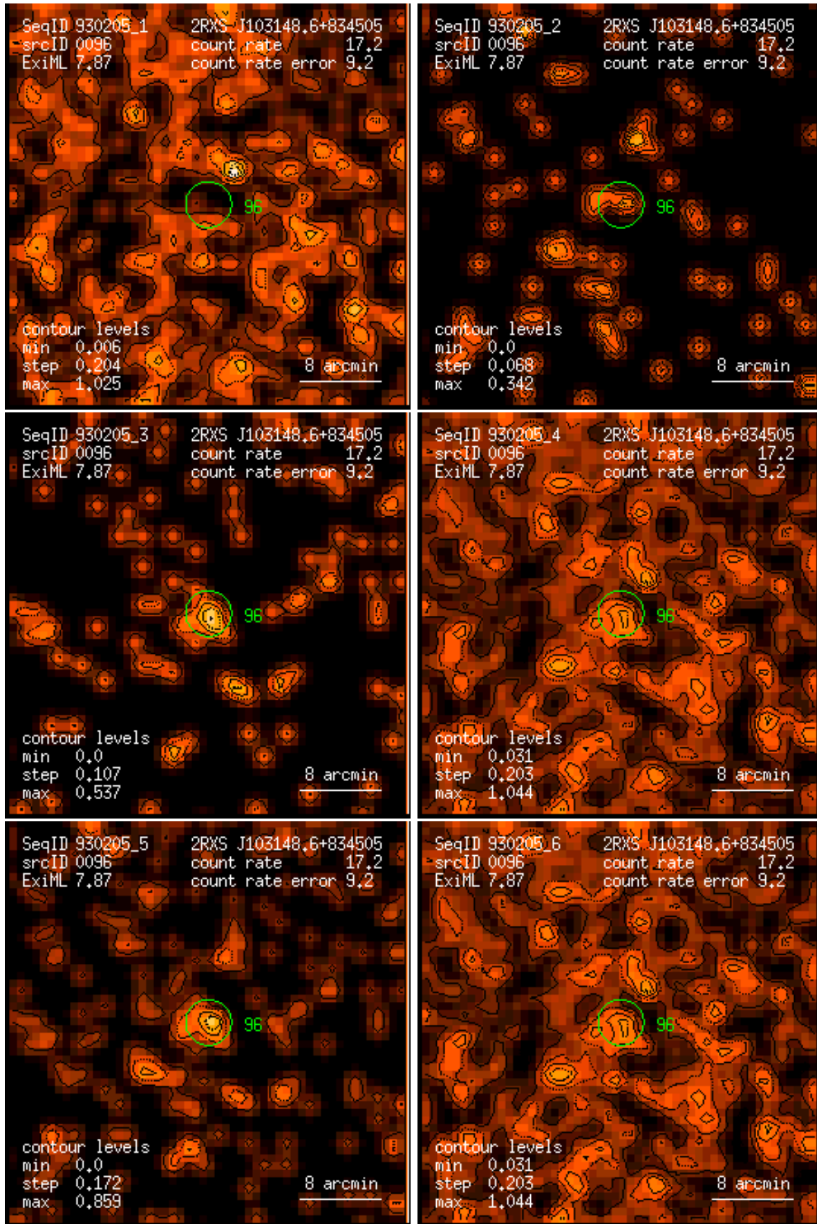
Figure 96: RASS 930205: detection 0096: band rate images, Gaussian filter: (1) PSPC channels 11 – 41, (2) 52 – 90, (3) 91 – 201, (4) 11 – 235, (5) 52 – 201, (6) 11 – 201. Broad band rates in counts/ks. Band rate contour levels in counts/ks/arcmin 2 .
