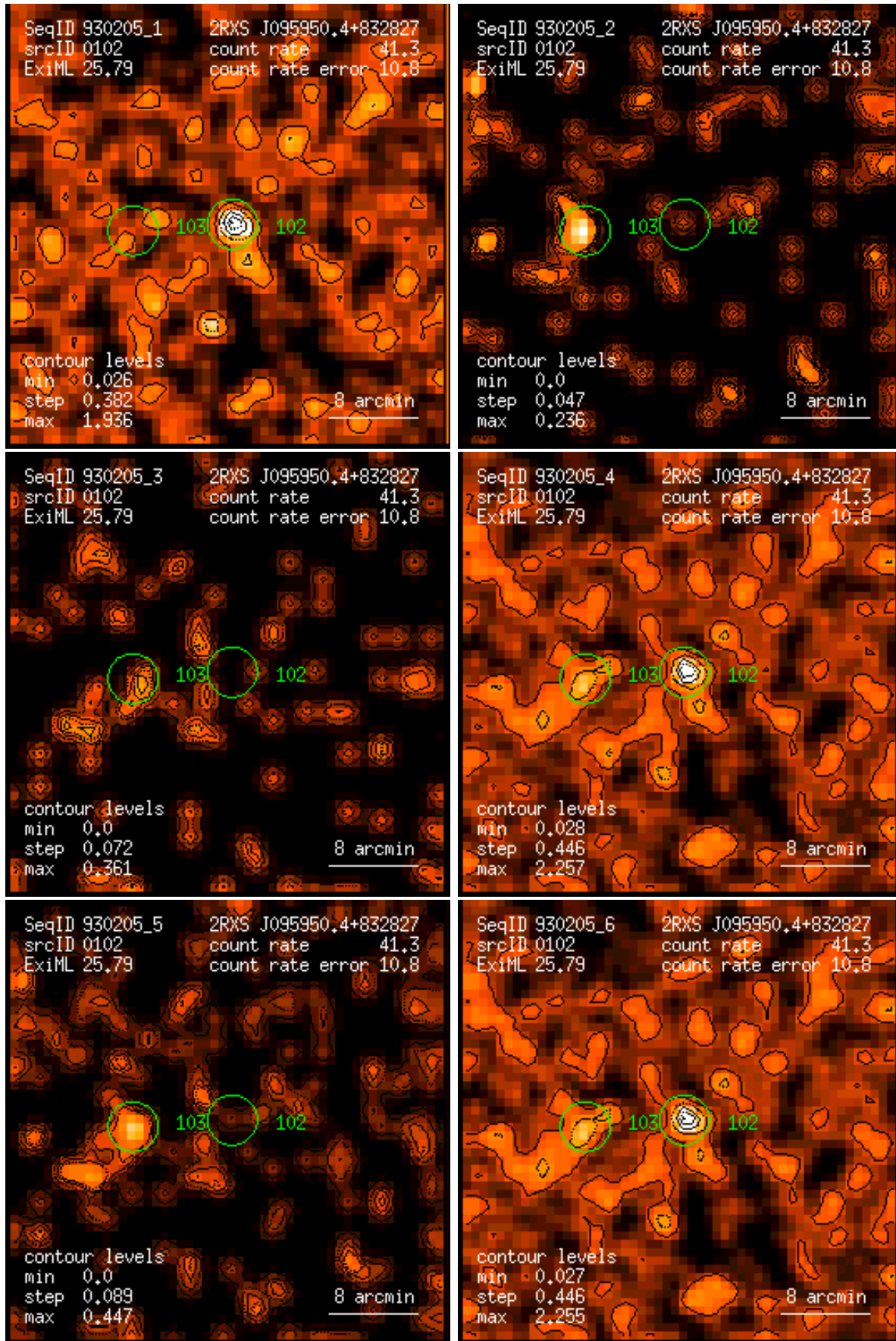
Figure 102: RASS 930205: detection 0102: band rate images, Gaussian filter: (1) PSPC channels 11 – 41, (2) 52 – 90, (3) 91 – 201, (4) 11 – 235, (5) 52 – 201, (6) 11 – 201. Broad band rates in counts/ks. Band rate contour levels in counts/ks/arcmin 2 .
