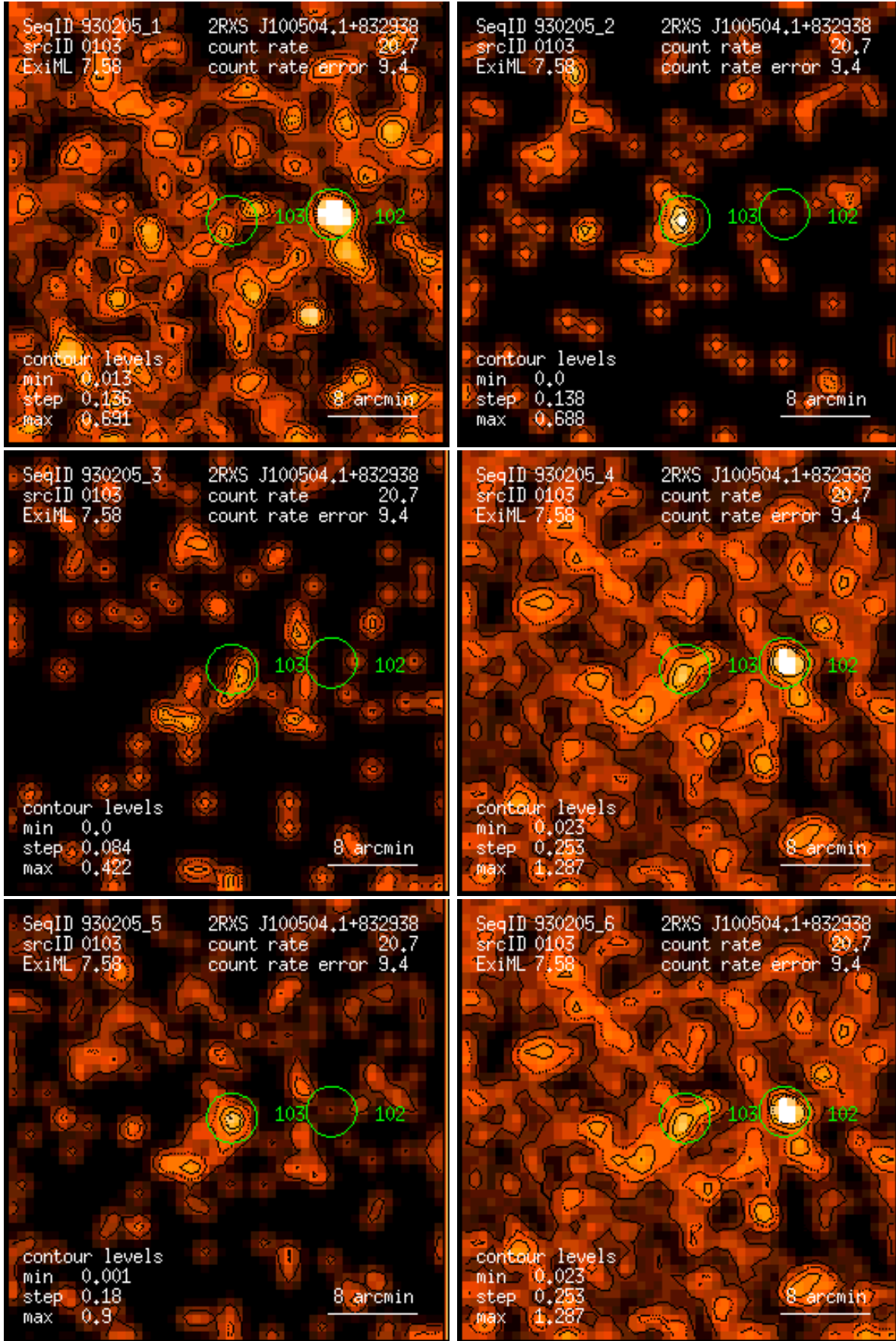
Figure 103: RASS 930205: detection 0103: band rate images, Gaussian filter: (1) PSPC channels 11 – 41, (2) 52 – 90, (3) 91 – 201, (4) 11 – 235, (5) 52 – 201, (6) 11 – 201. Broad band rates in counts/ks. Band rate contour levels in counts/ks/arcmin 2 .
