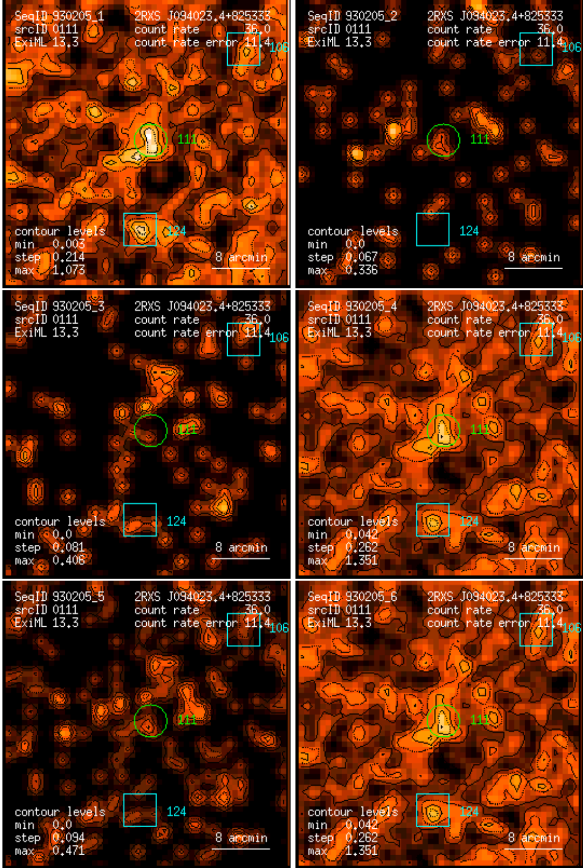
Figure 111: RASS 930205: detection 0111: band rate images, Gaussian filter: (1) PSPC channels 11 – 41, (2) 52 – 90, (3) 91 – 201, (4) 11 – 235, (5) 52 – 201, (6) 11 – 201. Broad band rates in counts/ks. Band rate contour levels in counts/ks/arcmin 2 .
