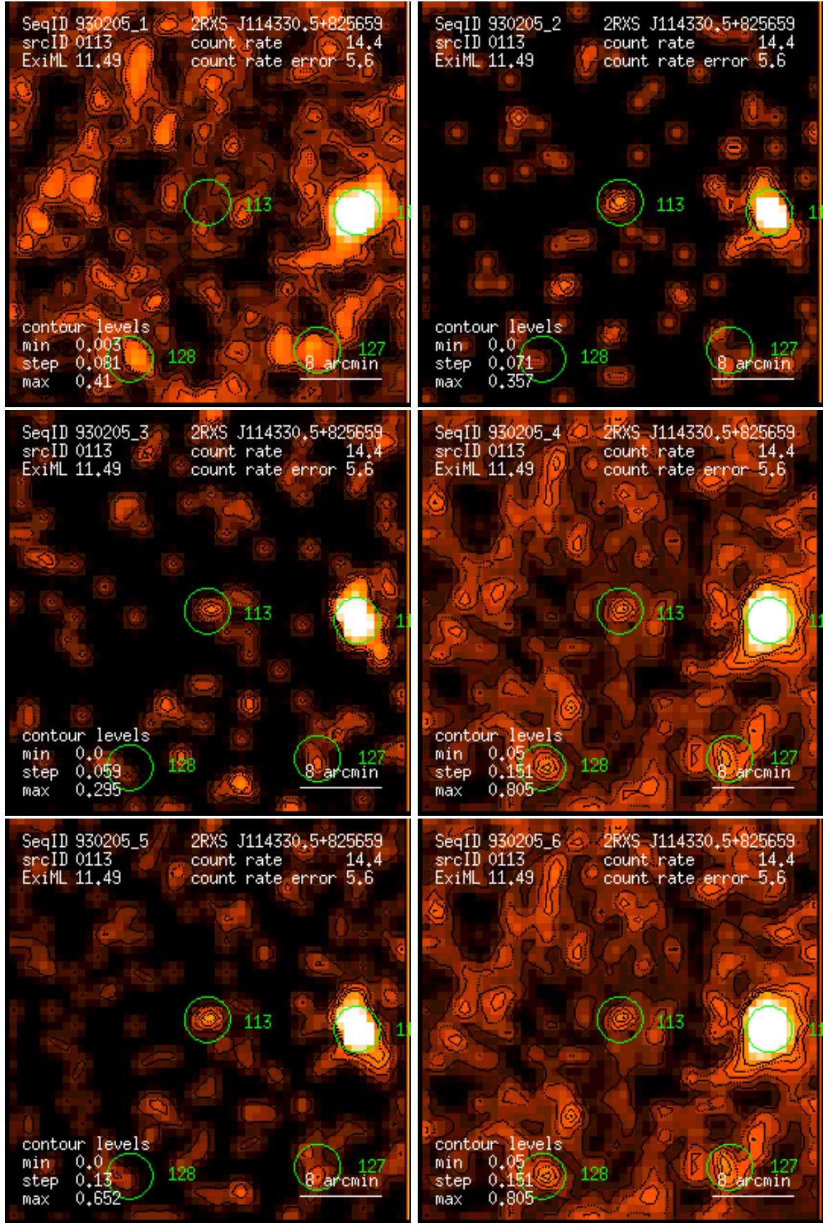
Figure 113: RASS 930205: detection 0113: band rate images, Gaussian filter: (1) PSPC channels 11 – 41, (2) 52 – 90, (3) 91 – 201, (4) 11 – 235, (5) 52 – 201, (6) 11 – 201. Broad band rates in counts/ks. Band rate contour levels in counts/ks/arcmin 2 .
