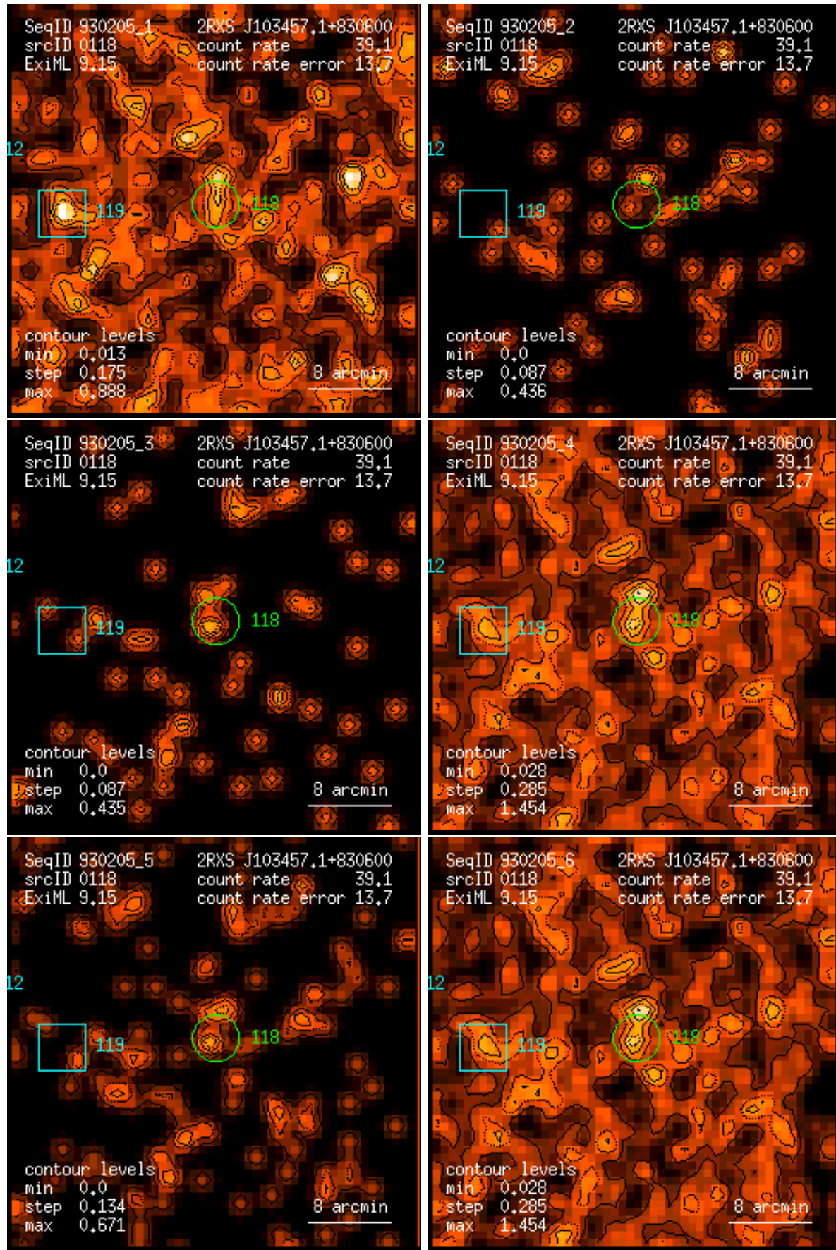
Figure 118: RASS 930205: detection 0118: band rate images, Gaussian filter: (1) PSPC channels 11 – 41, (2) 52 – 90, (3) 91 – 201, (4) 11 – 235, (5) 52 – 201, (6) 11 – 201. Broad band rates in counts/ks. Band rate contour levels in counts/ks/arcmin 2 .
