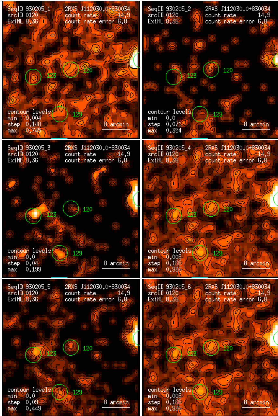
Figure 120: RASS 930205: detection 0120: band rate images, Gaussian filter: (1) PSPC channels 11 – 41, (2) 52 – 90, (3) 91 – 201, (4) 11 – 235, (5) 52 – 201, (6) 11 – 201. Broad band rates in counts/ks. Band rate contour levels in counts/ks/arcmin 2 .
