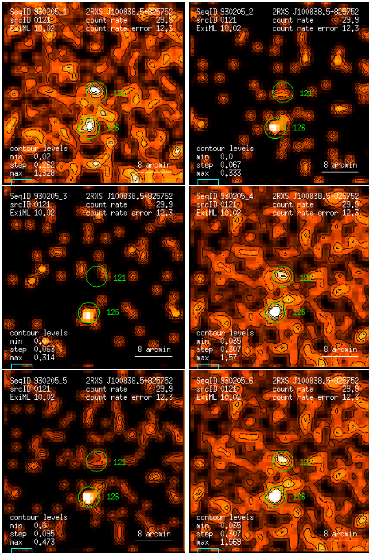
Figure 121: RASS 930205: detection 0121: band rate images, Gaussian filter: (1) PSPC channels 11 – 41, (2) 52 – 90, (3) 91 – 201, (4) 11 – 235, (5) 52 – 201, (6) 11 – 201. Broad band rates in counts/ks. Band rate contour levels in counts/ks/arcmin 2 .
