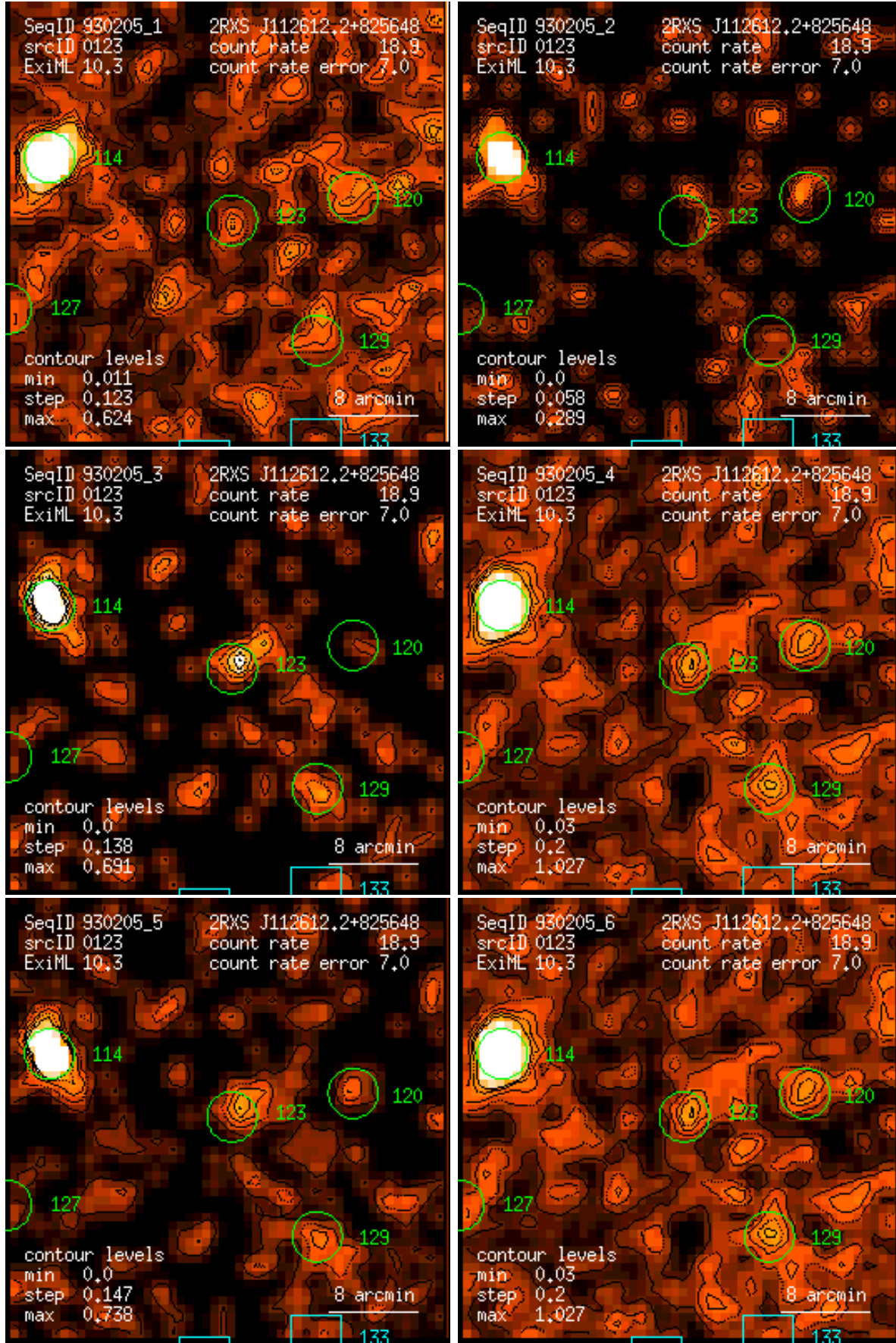
Figure 123: RASS 930205: detection 0123: band rate images, Gaussian filter: (1) PSPC channels 11 – 41, (2) 52 – 90, (3) 91 – 201, (4) 11 – 235, (5) 52 – 201, (6) 11 – 201. Broad band rates in counts/ks. Band rate contour levels in counts/ks/arcmin 2 .
