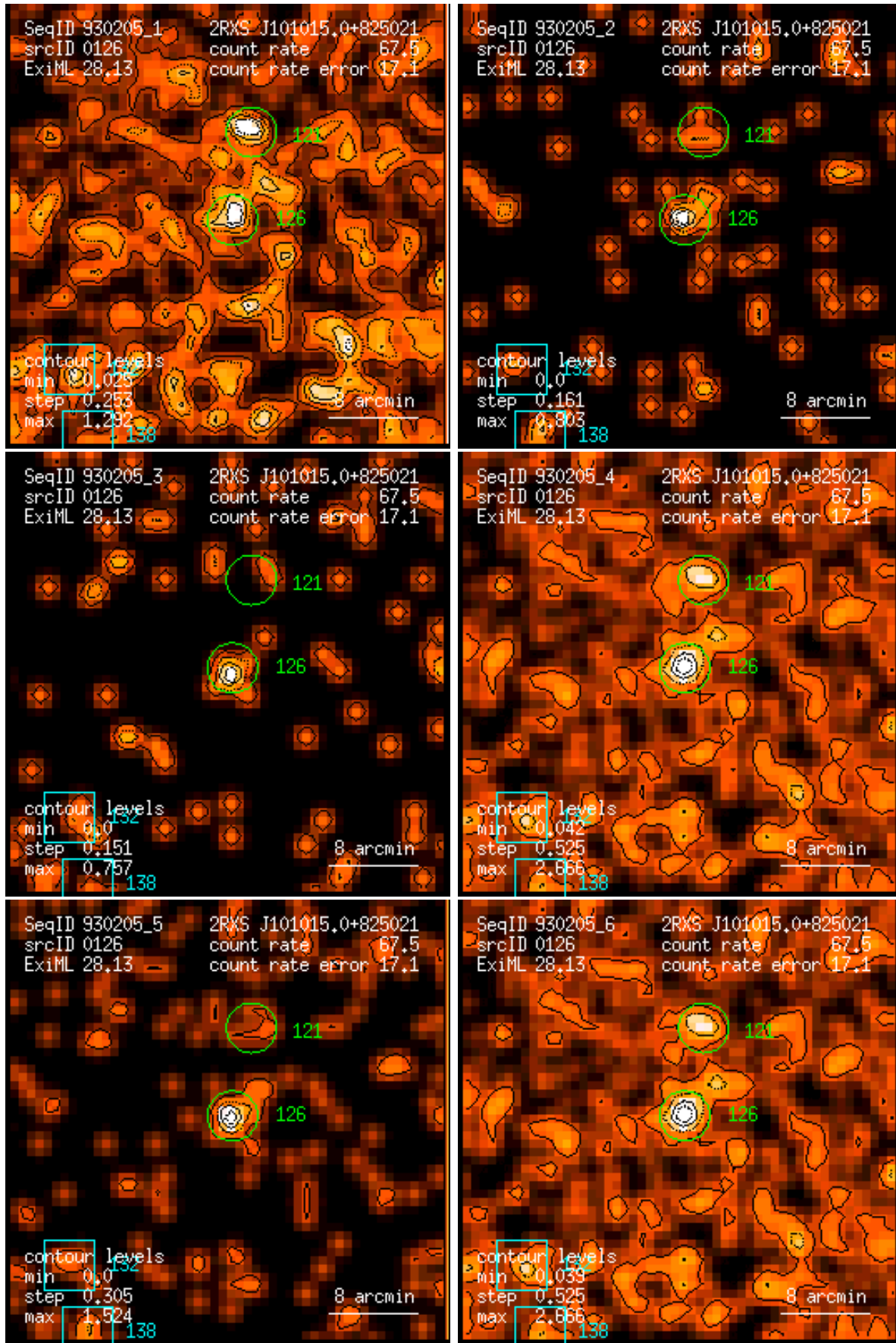
Figure 126: RASS 930205: detection 0126: band rate images, Gaussian filter: (1) PSPC channels 11 – 41, (2) 52 – 90, (3) 91 – 201, (4) 11 – 235, (5) 52 – 201, (6) 11 – 201. Broad band rates in counts/ks. Band rate contour levels in counts/ks/arcmin 2 .
