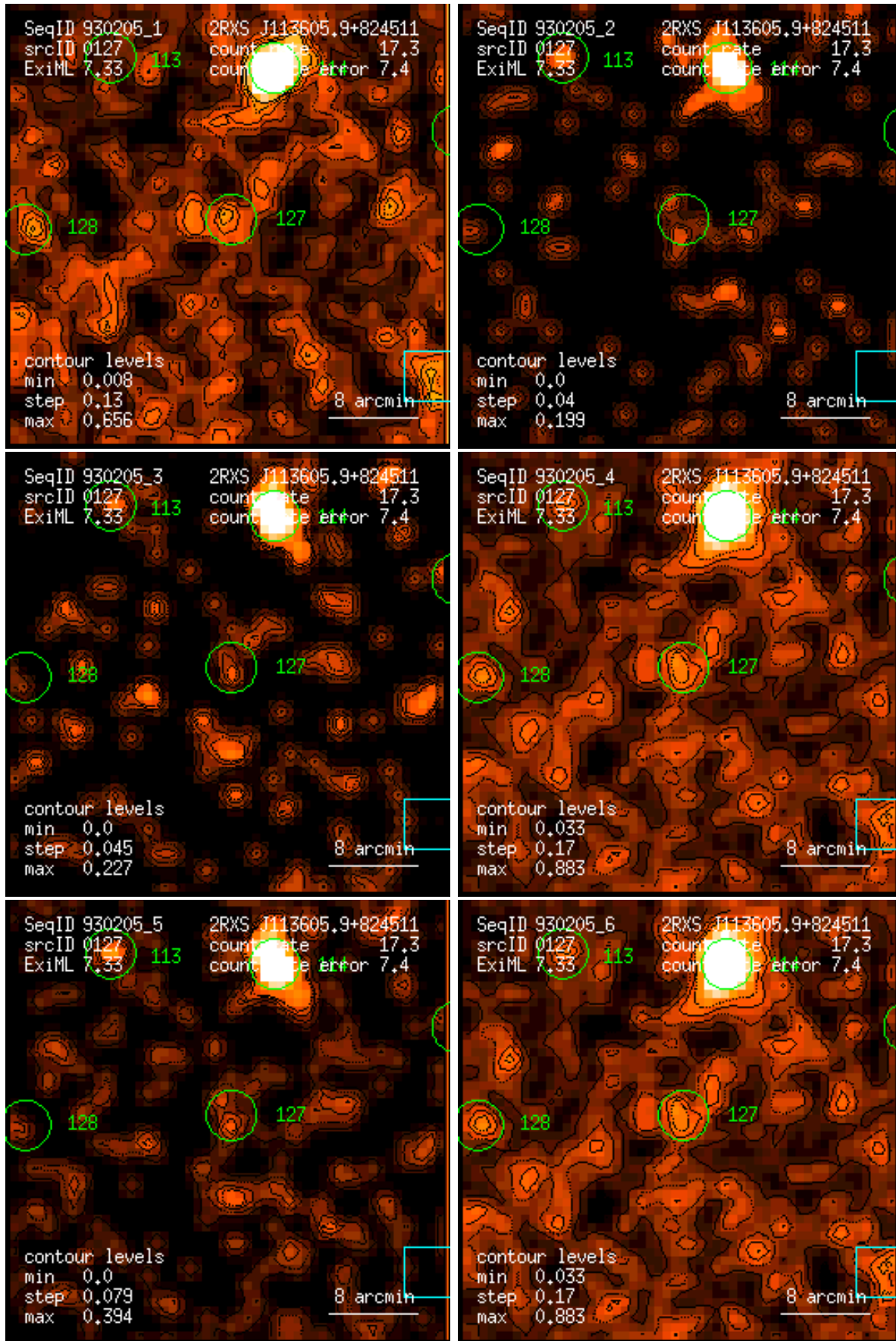
Figure 127: RASS 930205: detection 0127: band rate images, Gaussian filter: (1) PSPC channels 11 – 41, (2) 52 – 90, (3) 91 – 201, (4) 11 – 235, (5) 52 – 201, (6) 11 – 201. Broad band rates in counts/ks. Band rate contour levels in counts/ks/arcmin 2 .
