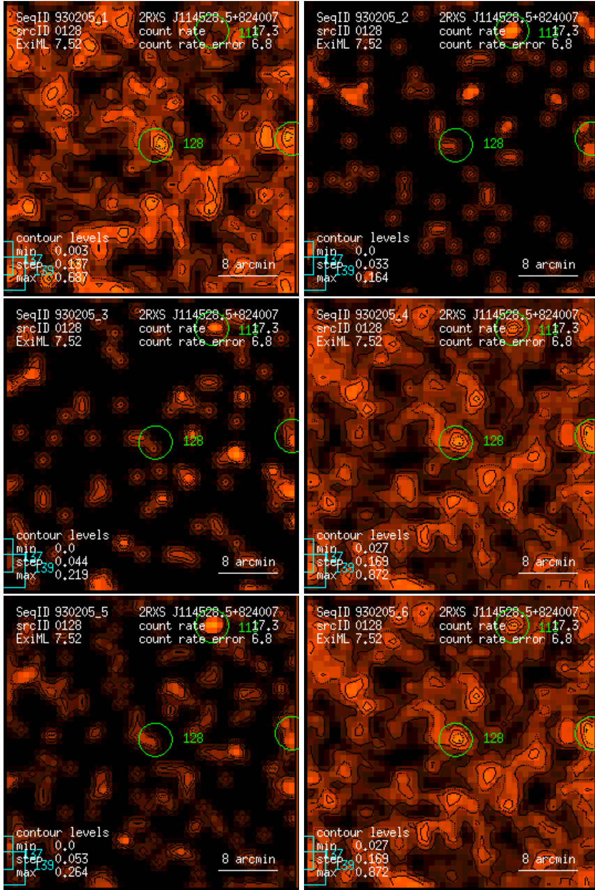
Figure 128: RASS 930205: detection 0128: band rate images, Gaussian filter: (1) PSPC channels 11 – 41, (2) 52 – 90, (3) 91 – 201, (4) 11 – 235, (5) 52 – 201, (6) 11 – 201. Broad band rates in counts/ks. Band rate contour levels in counts/ks/arcmin 2 .
