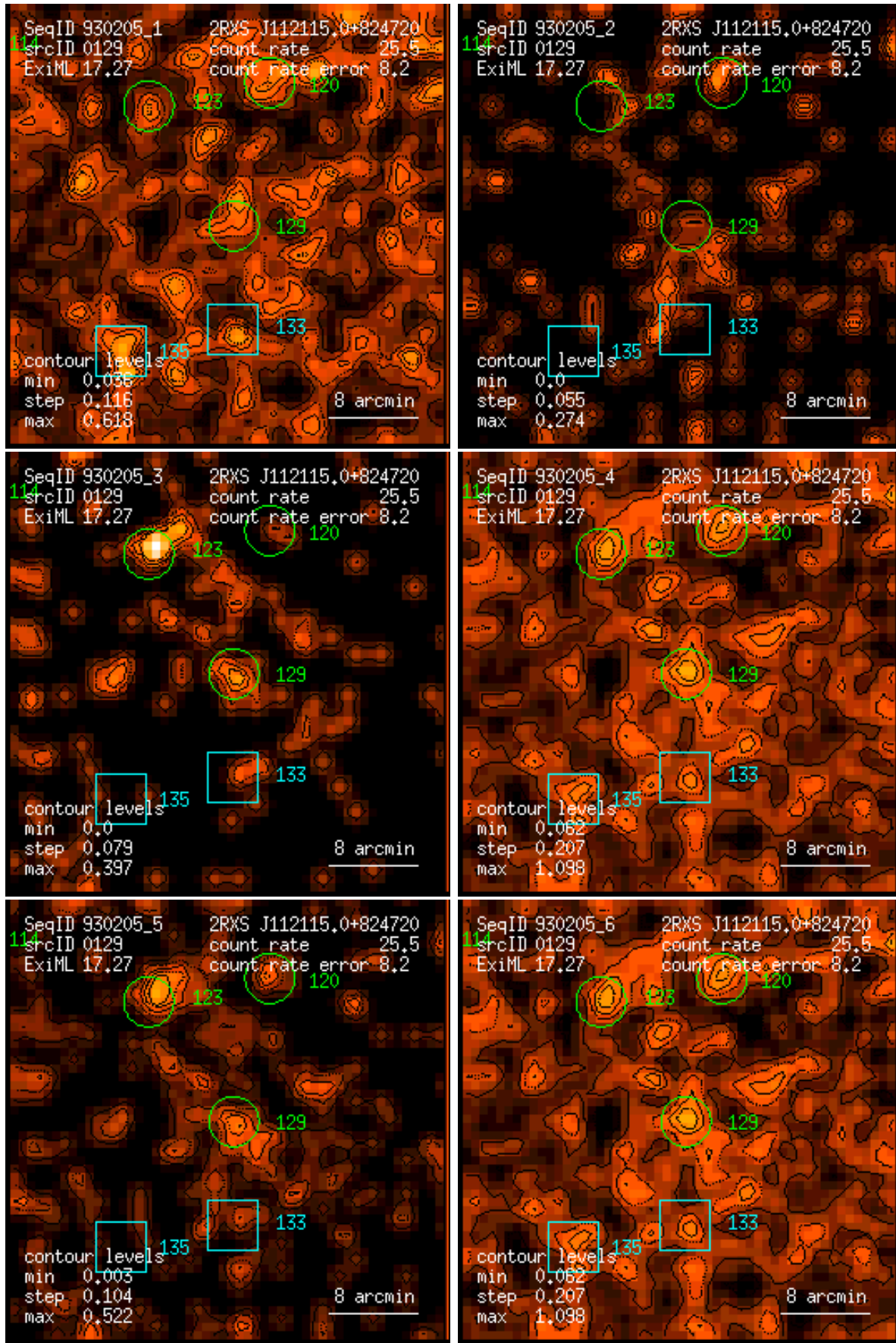
Figure 129: RASS 930205: detection 0129: band rate images, Gaussian filter: (1) PSPC channels 11 – 41, (2) 52 – 90, (3) 91 – 201, (4) 11 – 235, (5) 52 – 201, (6) 11 – 201. Broad band rates in counts/ks. Band rate contour levels in counts/ks/arcmin 2 .
