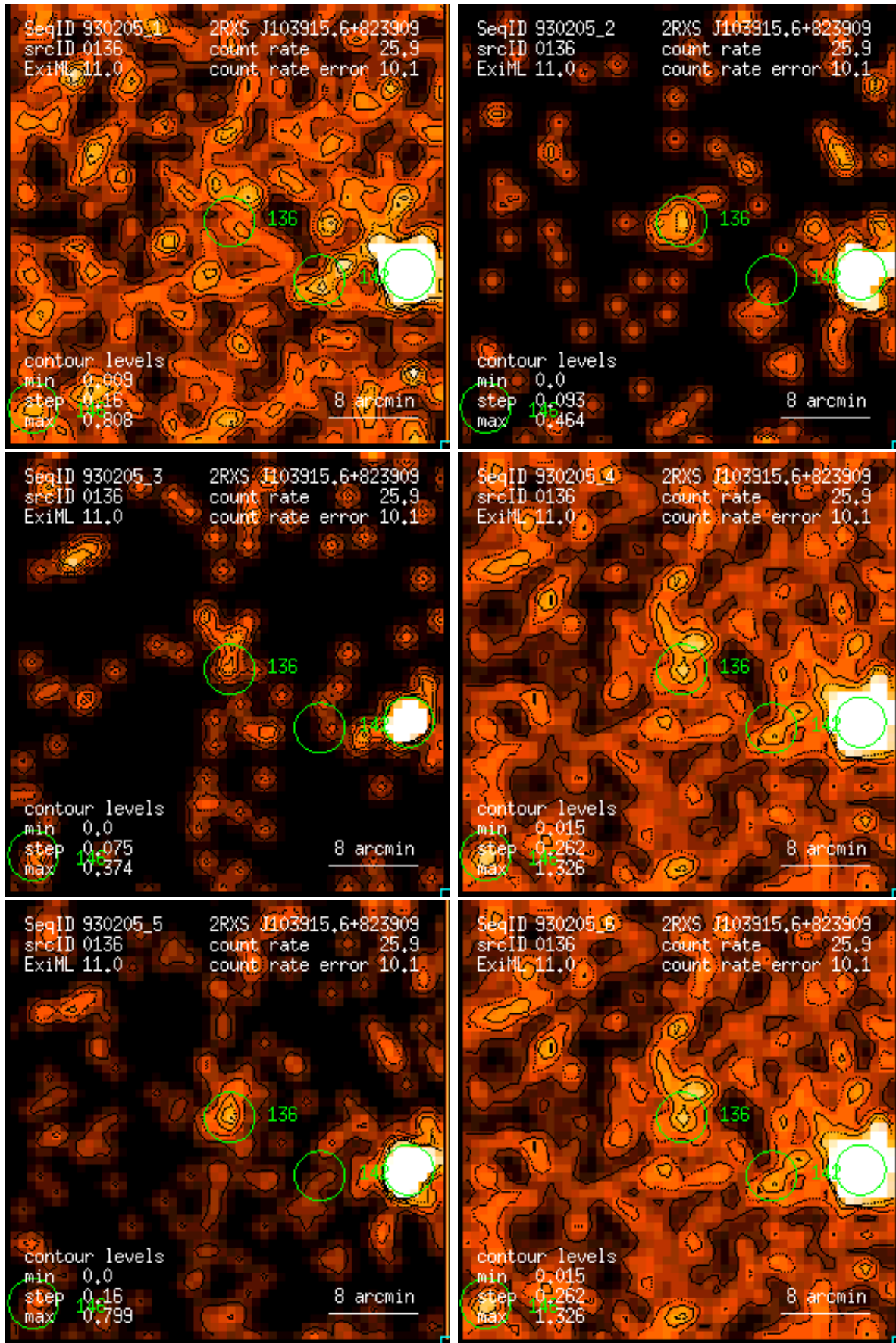
Figure 136: RASS 930205: detection 0136: band rate images, Gaussian filter: (1) PSPC channels 11 – 41, (2) 52 – 90, (3) 91 – 201, (4) 11 – 235, (5) 52 – 201, (6) 11 – 201. Broad band rates in counts/ks. Band rate contour levels in counts/ks/arcmin 2 .
