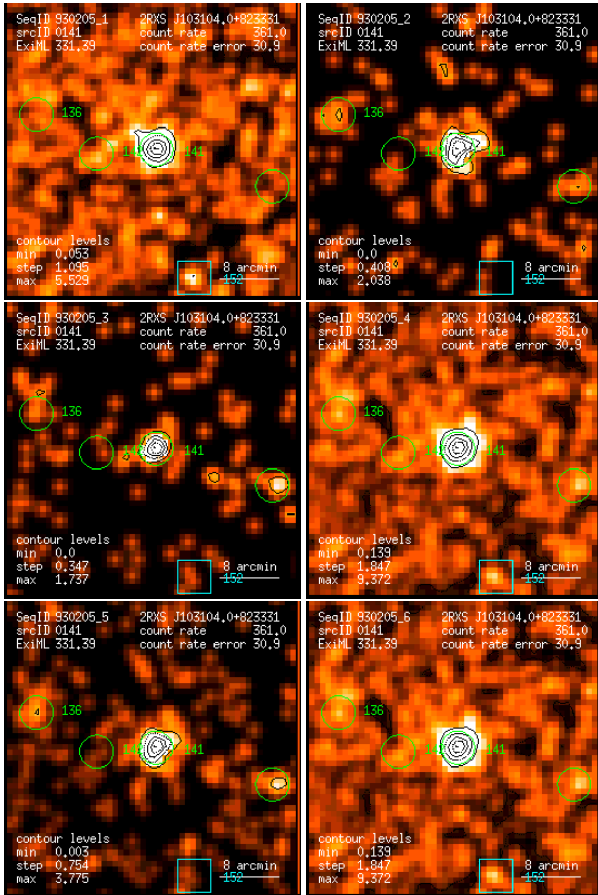
Figure 141: RASS 930205: detection 0141: band rate images, Gaussian filter: (1) PSPC channels 11 – 41, (2) 52 – 90, (3) 91 – 201, (4) 11 – 235, (5) 52 – 201, (6) 11 – 201. Broad band rates in counts/ks. Band rate contour levels in counts/ks/arcmin 2 .
