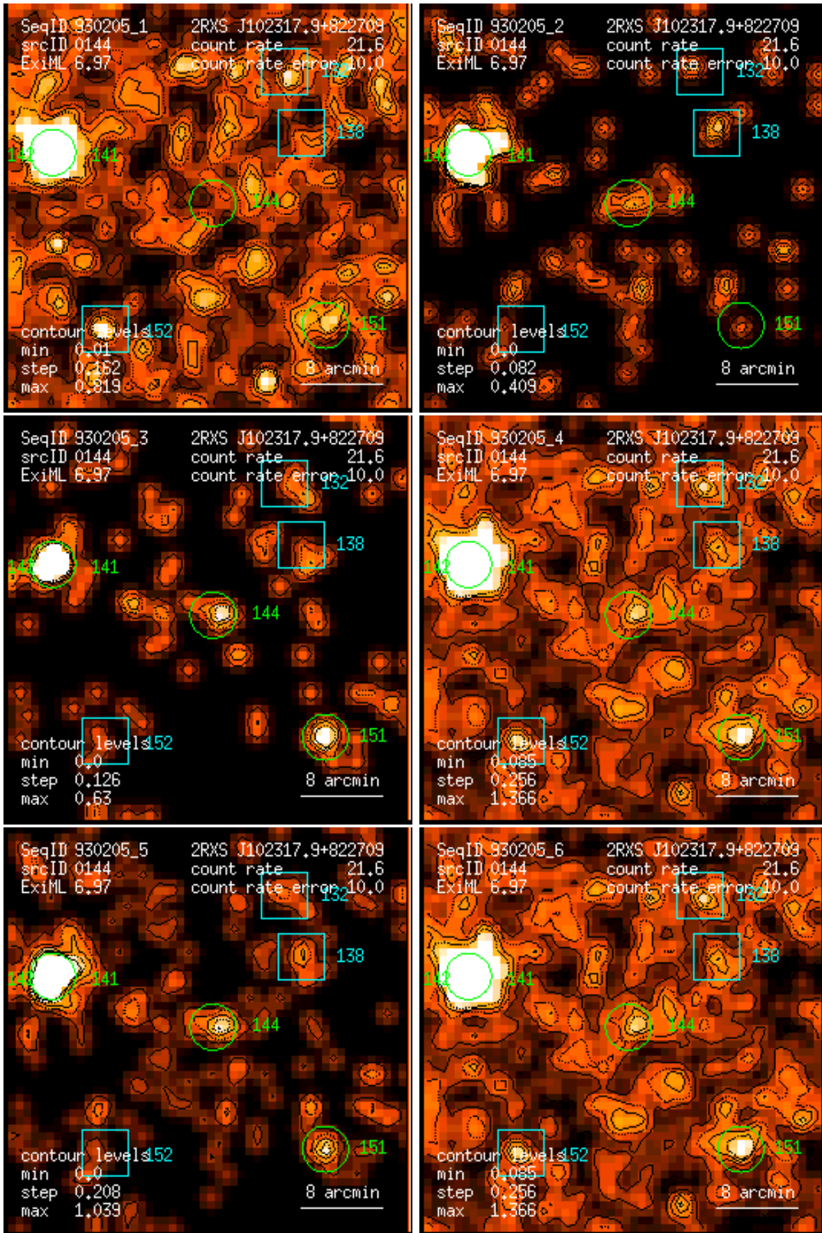
Figure 144: RASS 930205: detection 0144: band rate images, Gaussian filter: (1) PSPC channels 11 – 41, (2) 52 – 90, (3) 91 – 201, (4) 11 – 235, (5) 52 – 201, (6) 11 – 201. Broad band rates in counts/ks. Band rate contour levels in counts/ks/arcmin 2 .
