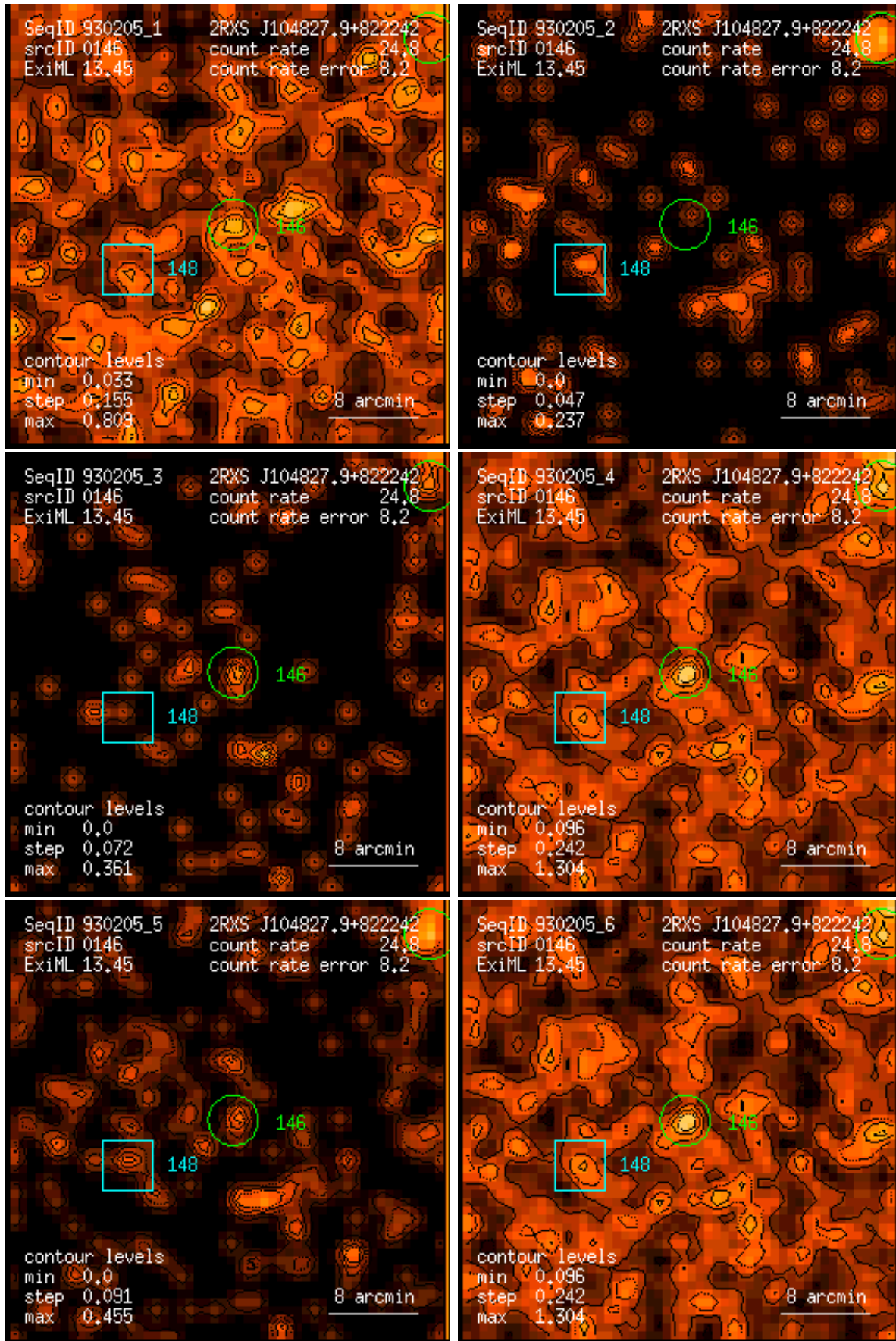
Figure 146: RASS 930205: detection 0146: band rate images, Gaussian filter: (1) PSPC channels 11 – 41, (2) 52 – 90, (3) 91 – 201, (4) 11 – 235, (5) 52 – 201, (6) 11 – 201. Broad band rates in counts/ks. Band rate contour levels in counts/ks/arcmin 2 .
