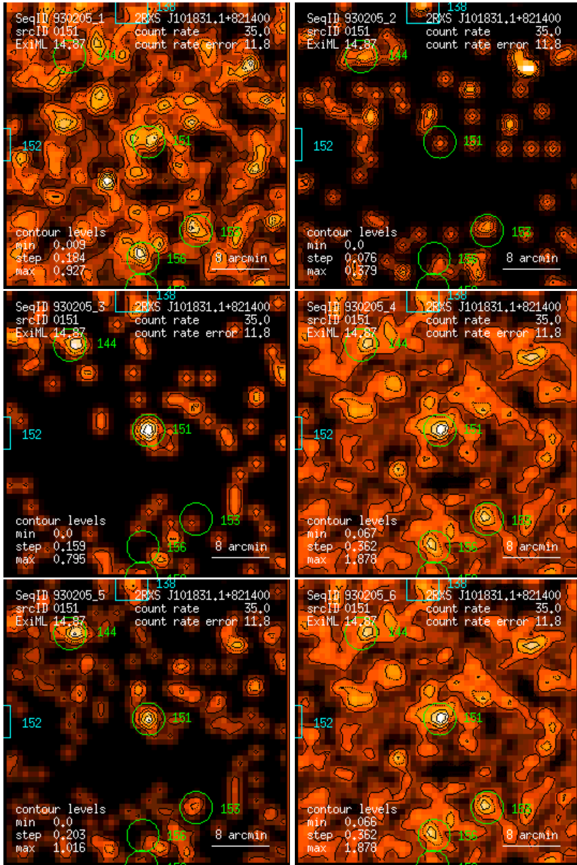
Figure 151: RASS 930205: detection 0151: band rate images, Gaussian filter: (1) PSPC channels 11 – 41, (2) 52 – 90, (3) 91 – 201, (4) 11 – 235, (5) 52 – 201, (6) 11 – 201. Broad band rates in counts/ks. Band rate contour levels in counts/ks/arcmin 2 .
