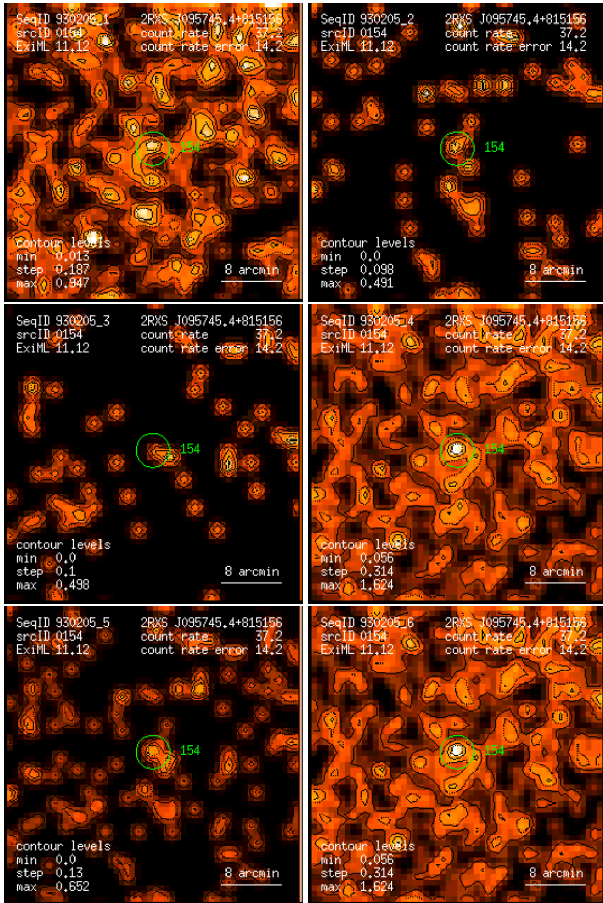
Figure 154: RASS 930205: detection 0154: band rate images, Gaussian filter: (1) PSPC channels 11 – 41, (2) 52 – 90, (3) 91 – 201, (4) 11 – 235, (5) 52 – 201, (6) 11 – 201. Broad band rates in counts/ks. Band rate contour levels in counts/ks/arcmin 2 .
