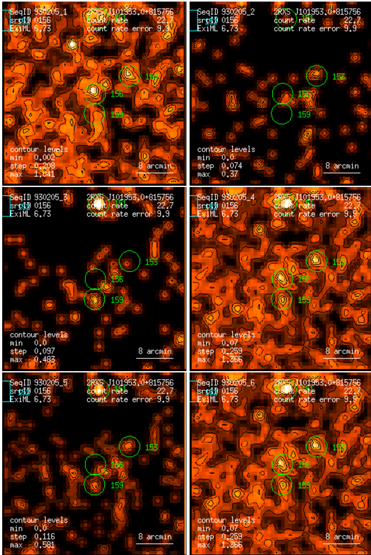
Figure 156: RASS 930205: detection 0156: band rate images, Gaussian filter: (1) PSPC channels 11 – 41, (2) 52 – 90, (3) 91 – 201, (4) 11 – 235, (5) 52 – 201, (6) 11 – 201. Broad band rates in counts/ks. Band rate contour levels in counts/ks/arcmin 2 .
