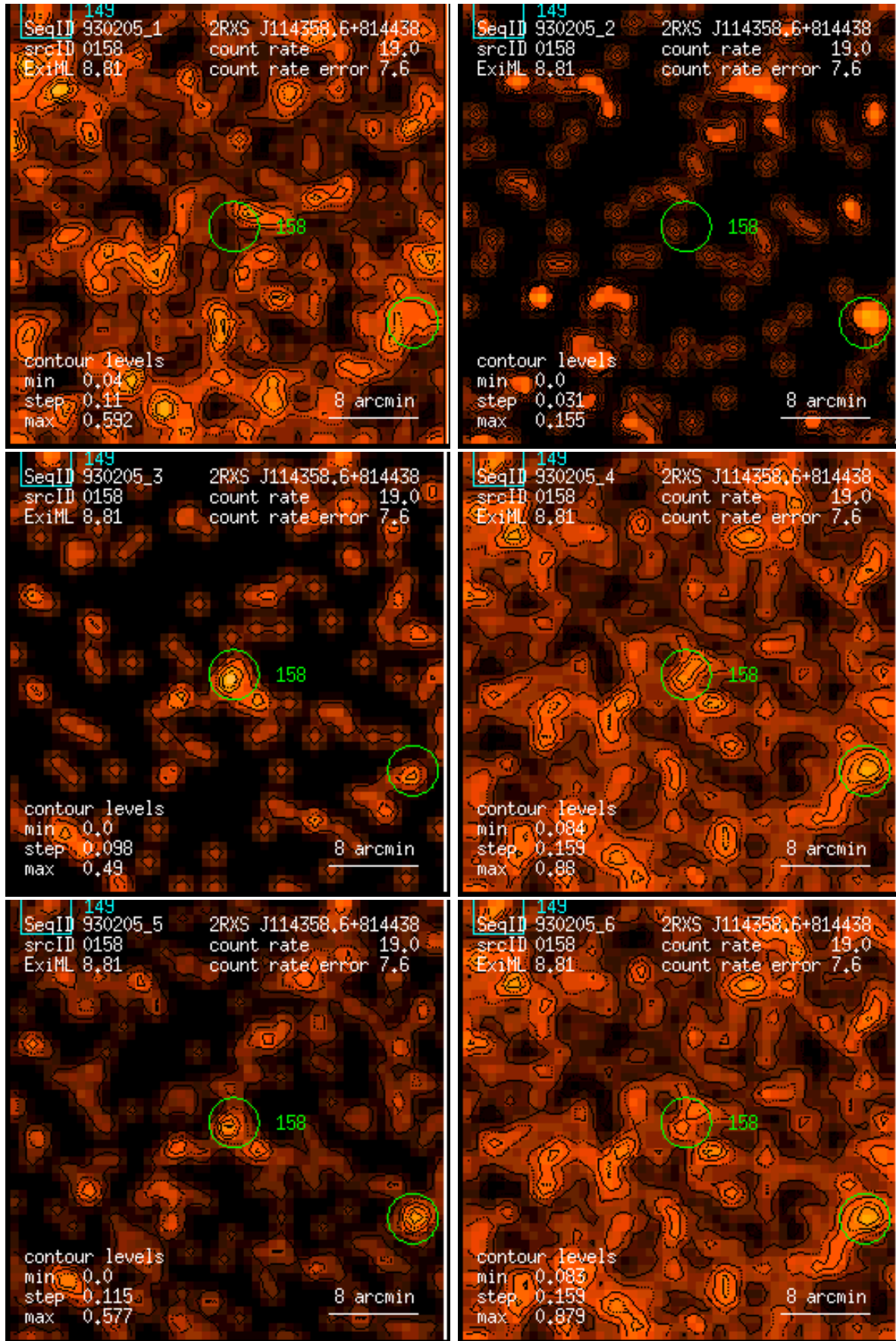
Figure 158: RASS 930205: detection 0158: band rate images, Gaussian filter: (1) PSPC channels 11 – 41, (2) 52 – 90, (3) 91 – 201, (4) 11 – 235, (5) 52 – 201, (6) 11 – 201. Broad band rates in counts/ks. Band rate contour levels in counts/ks/arcmin 2 .
