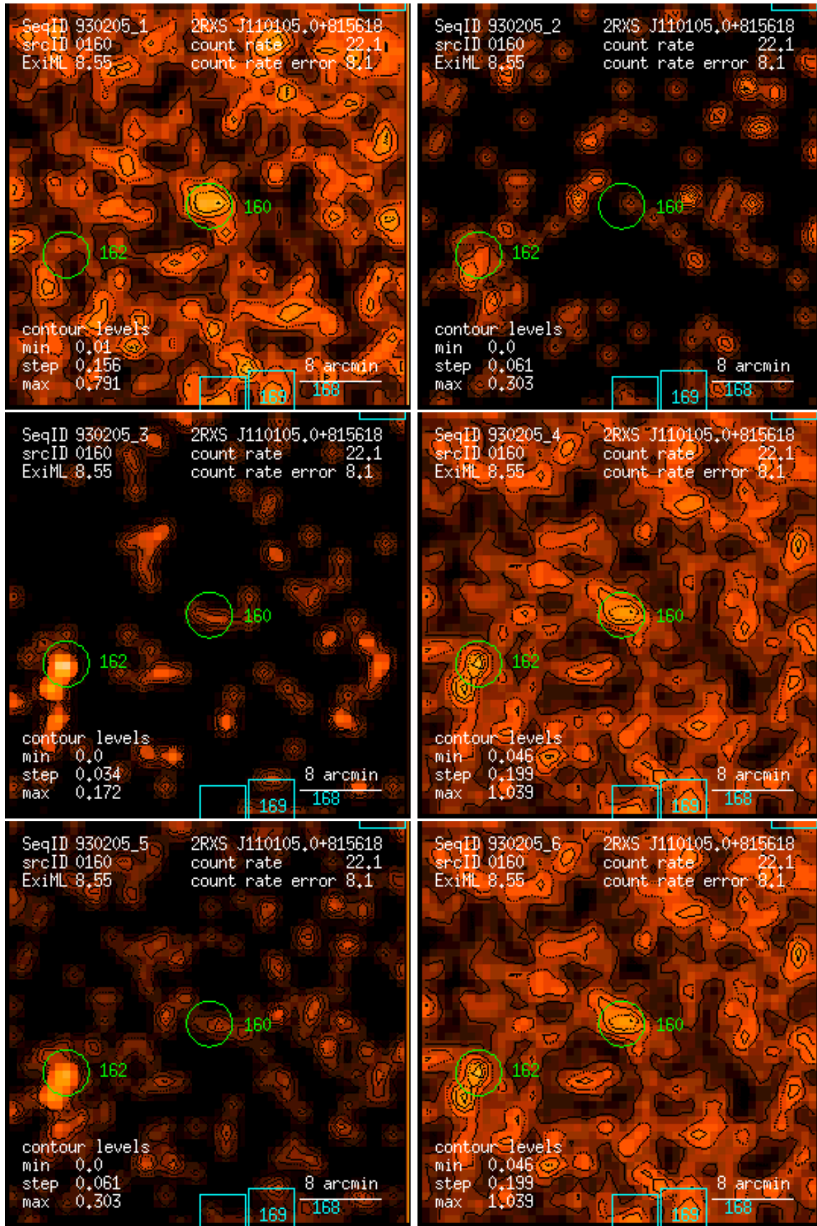
Figure 160: RASS 930205: detection 0160: band rate images, Gaussian filter: (1) PSPC channels 11 – 41, (2) 52 – 90, (3) 91 – 201, (4) 11 – 235, (5) 52 – 201, (6) 11 – 201. Broad band rates in counts/ks. Band rate contour levels in counts/ks/arcmin 2 .
