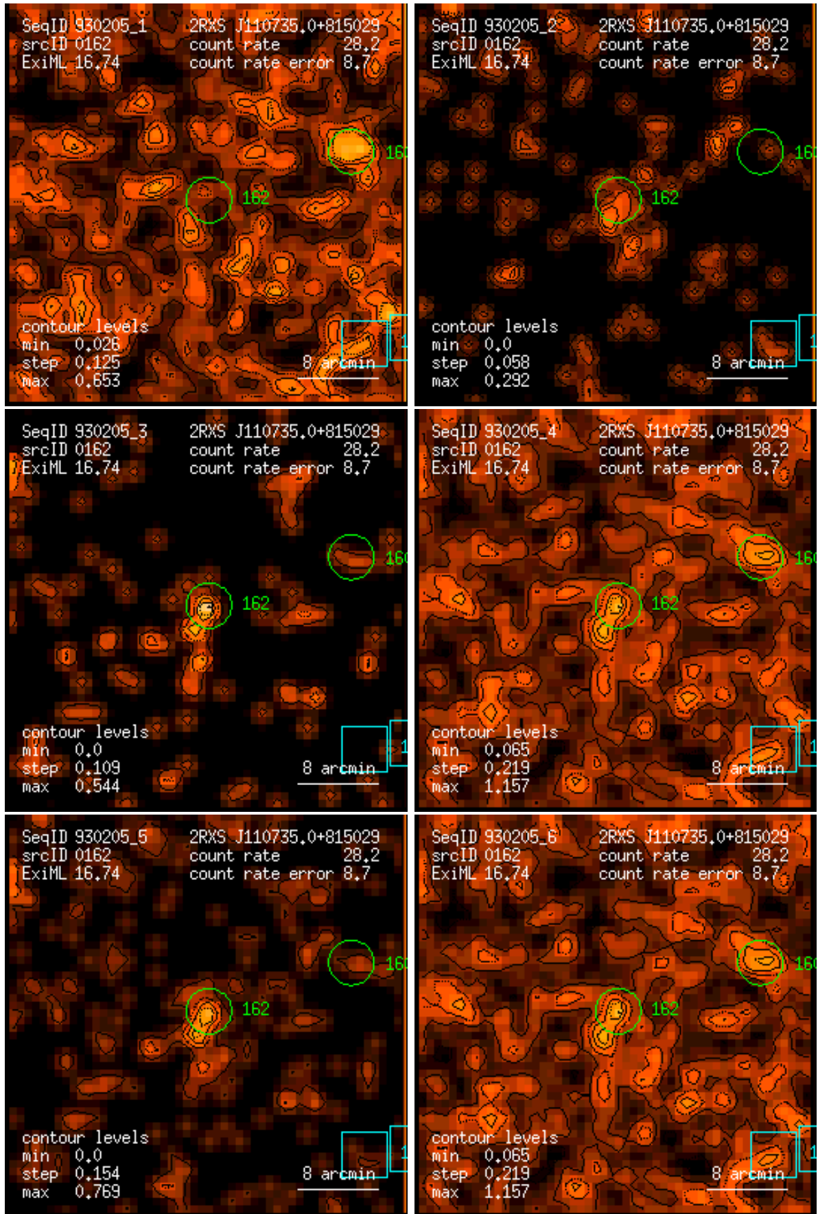
Figure 162: RASS 930205: detection 0162: band rate images, Gaussian filter: (1) PSPC channels 11 – 41, (2) 52 – 90, (3) 91 – 201, (4) 11 – 235, (5) 52 – 201, (6) 11 – 201. Broad band rates in counts/ks. Band rate contour levels in counts/ks/arcmin 2 .
