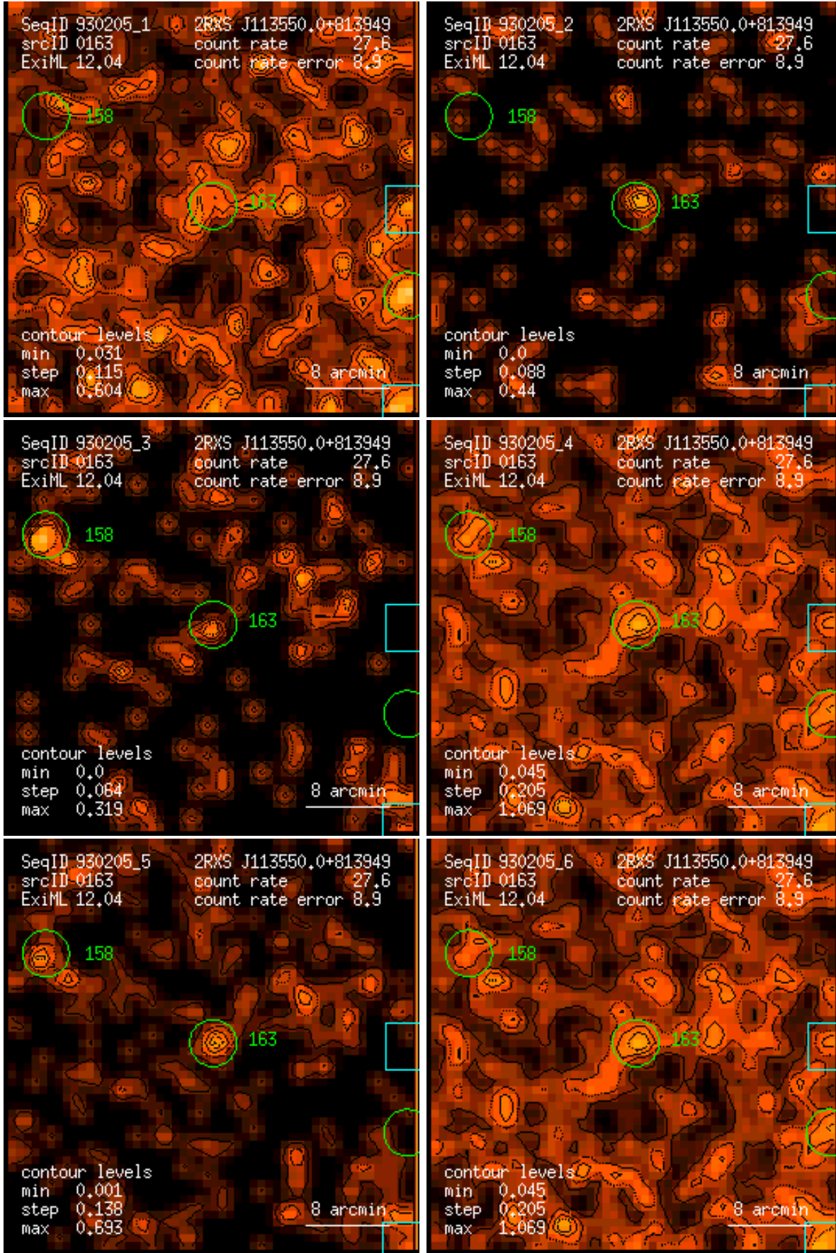
Figure 163: RASS 930205: detection 0163: band rate images, Gaussian filter: (1) PSPC channels 11 – 41, (2) 52 – 90, (3) 91 – 201, (4) 11 – 235, (5) 52 – 201, (6) 11 – 201. Broad band rates in counts/ks. Band rate contour levels in counts/ks/arcmin 2 .
