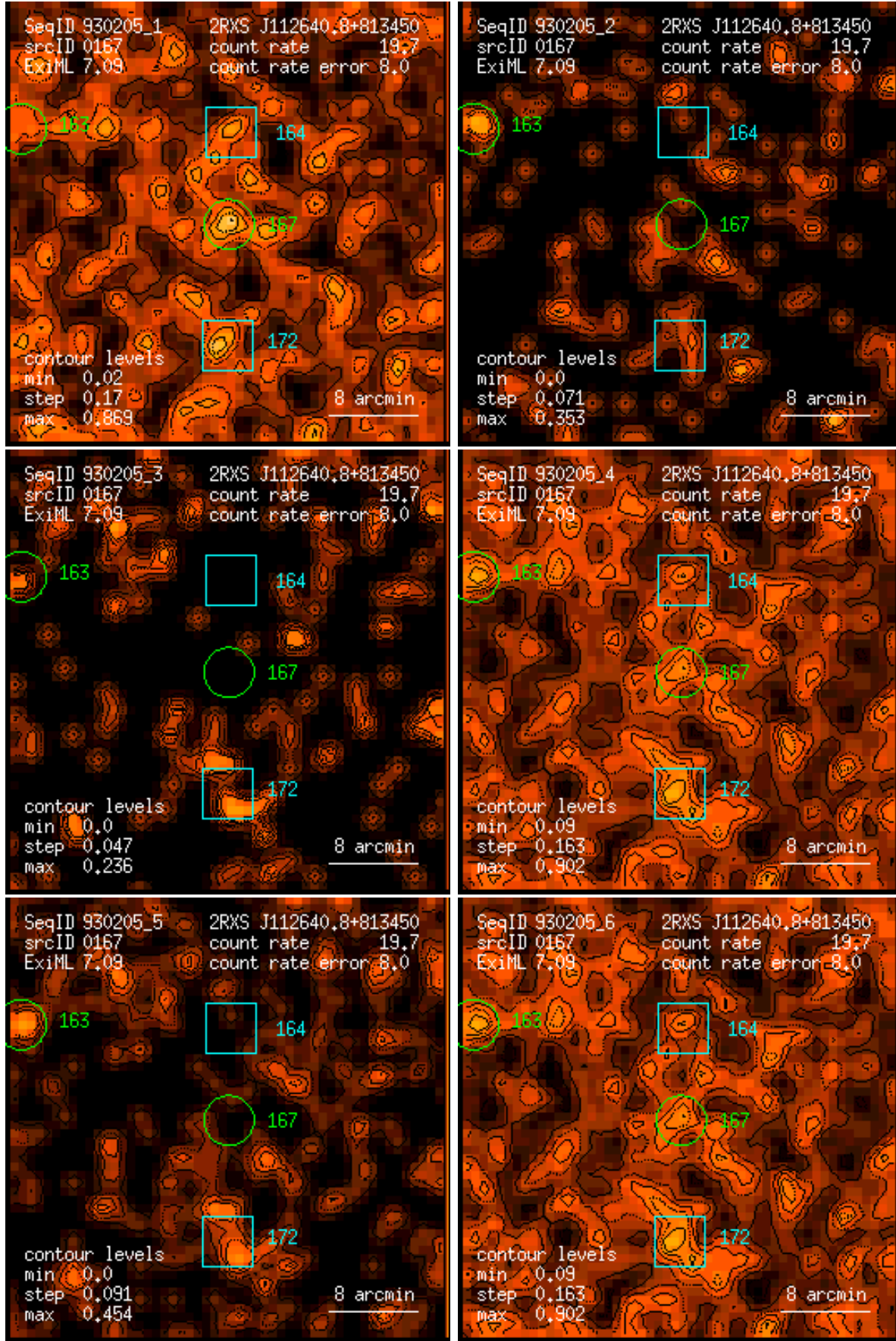
Figure 167: RASS 930205: detection 0167: band rate images, Gaussian filter: (1) PSPC channels 11 – 41, (2) 52 – 90, (3) 91 – 201, (4) 11 – 235, (5) 52 – 201, (6) 11 – 201. Broad band rates in counts/ks. Band rate contour levels in counts/ks/arcmin 2 .
