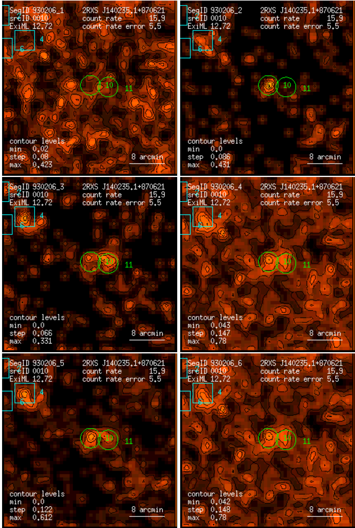
Figure 10: RASS 930206: detection 0010: band rate images, Gaussian filter: (1) PSPC channels 11 – 41, (2) 52 – 90, (3) 91 – 201, (4) 11 – 235, (5) 52 – 201, (6) 11 – 201. Broad band rates in counts/ks. Band rate contour levels in counts/ks/arcmin 2 .
