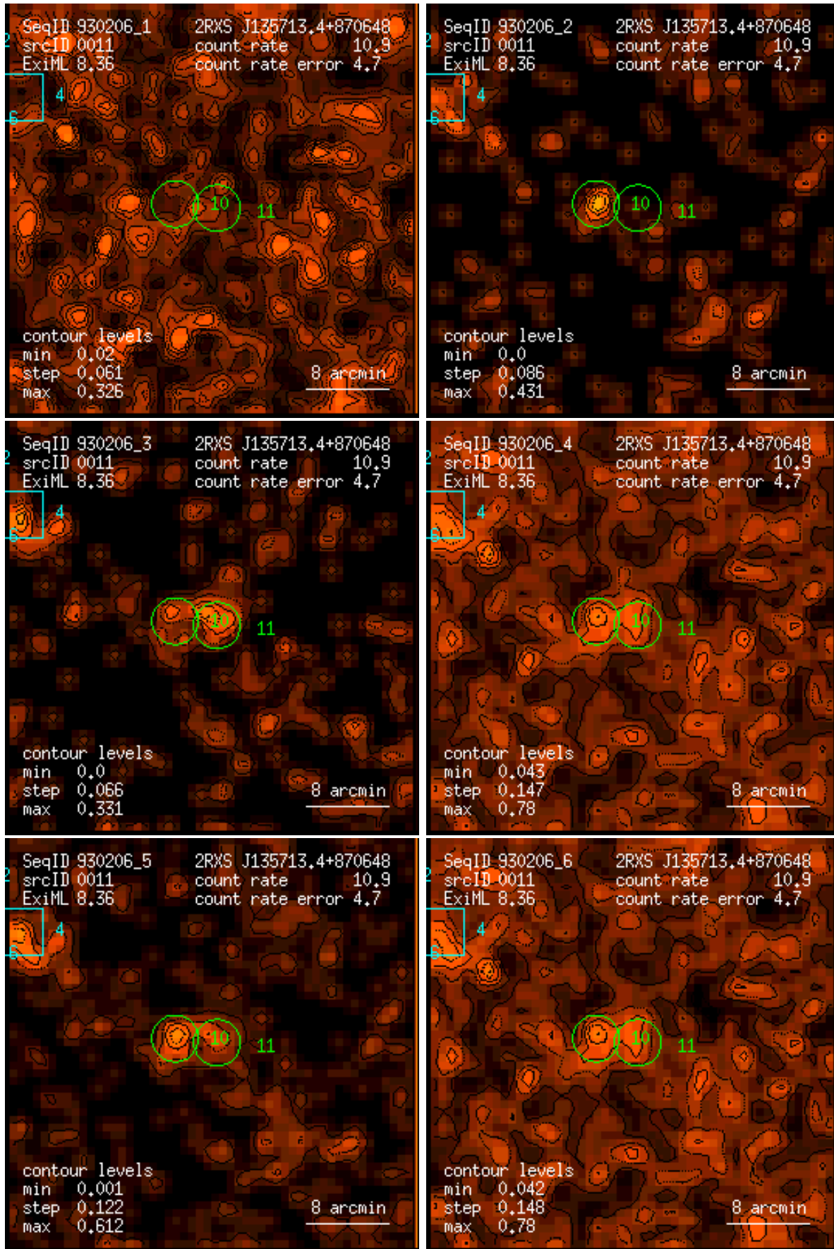
Figure 11: RASS 930206: detection 0011: band rate images, Gaussian filter: (1) PSPC channels 11 – 41, (2) 52 – 90, (3) 91 – 201, (4) 11 – 235, (5) 52 – 201, (6) 11 – 201. Broad band rates in counts/ks. Band rate contour levels in counts/ks/arcmin 2 .
