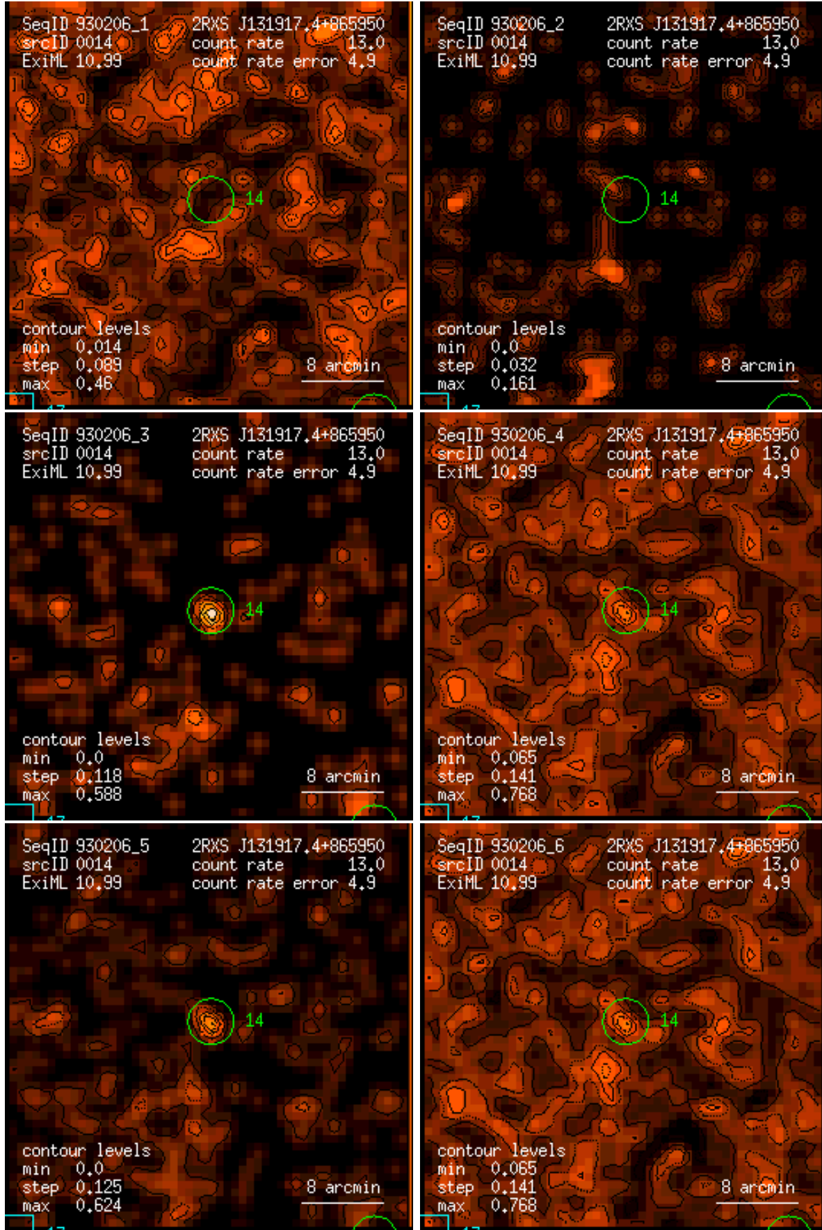
Figure 14: RASS 930206: detection 0014: band rate images, Gaussian filter: (1) PSPC channels 11 – 41, (2) 52 – 90, (3) 91 – 201, (4) 11 – 235, (5) 52 – 201, (6) 11 – 201. Broad band rates in counts/ks. Band rate contour levels in counts/ks/arcmin 2 .
