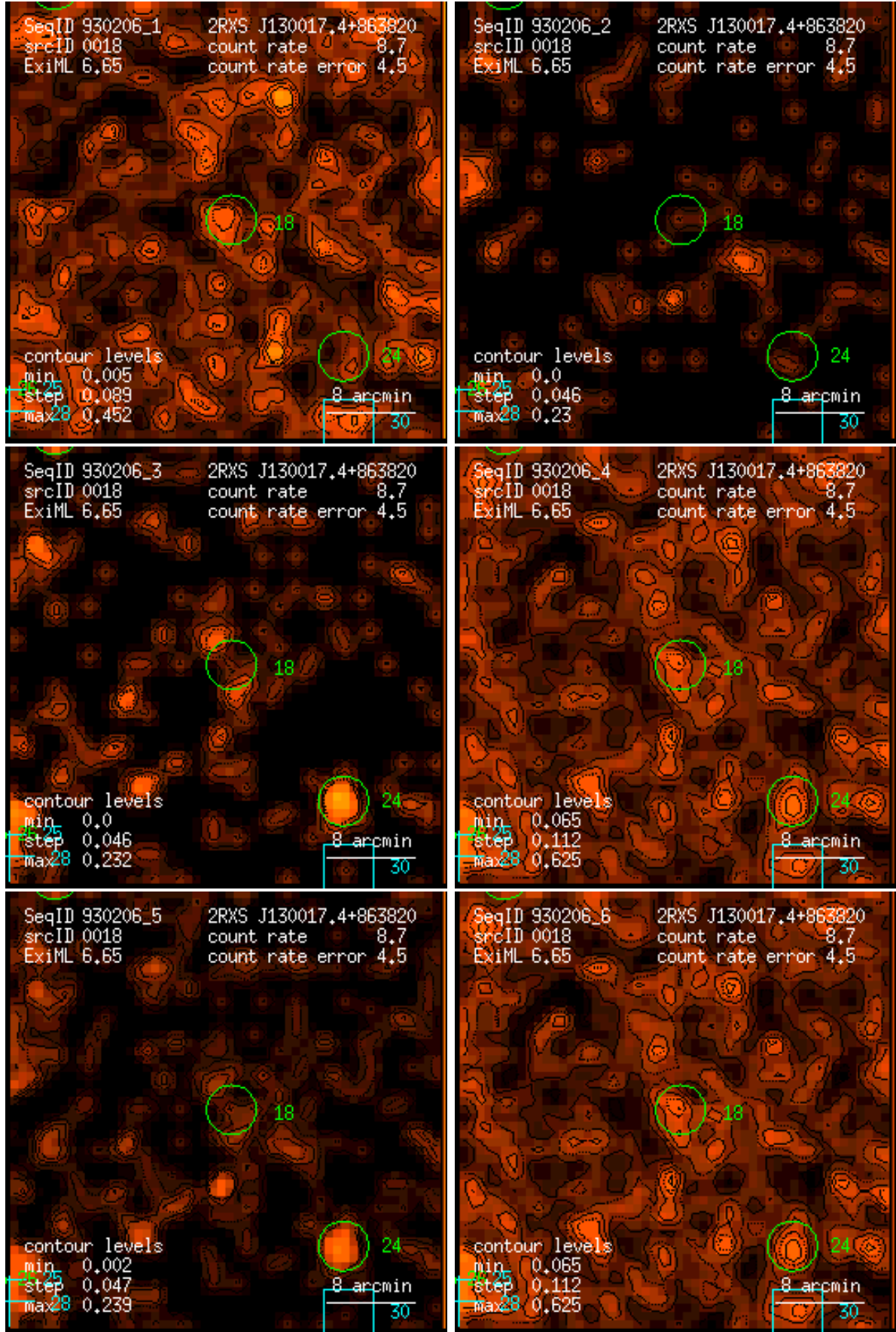
Figure 18: RASS 930206: detection 0018: band rate images, Gaussian filter: (1) PSPC channels 11 – 41, (2) 52 – 90, (3) 91 – 201, (4) 11 – 235, (5) 52 – 201, (6) 11 – 201. Broad band rates in counts/ks. Band rate contour levels in counts/ks/arcmin 2 .
