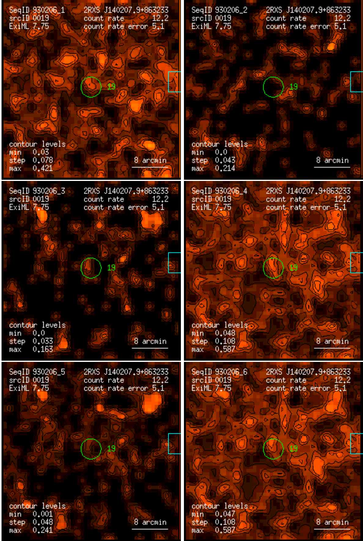
Figure 19: RASS 930206: detection 0019: band rate images, Gaussian filter: (1) PSPC channels 11 – 41, (2) 52 – 90, (3) 91 – 201, (4) 11 – 235, (5) 52 – 201, (6) 11 – 201. Broad band rates in counts/ks. Band rate contour levels in counts/ks/arcmin 2 .
