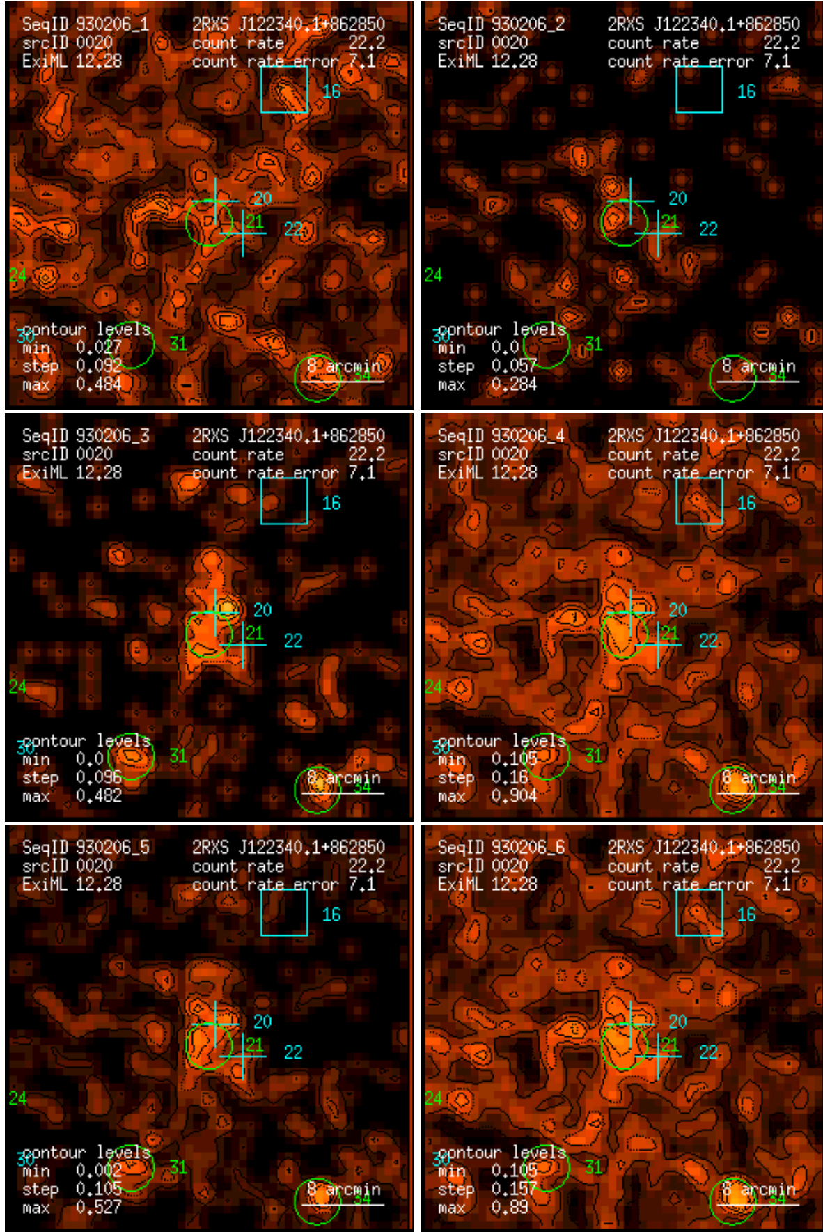
Figure 20: RASS 930206: detection 0020: band rate images, Gaussian filter: (1) PSPC channels 11 – 41, (2) 52 – 90, (3) 91 – 201, (4) 11 – 235, (5) 52 – 201, (6) 11 – 201. Broad band rates in counts/ks. Band rate contour levels in counts/ks/arcmin 2 .
