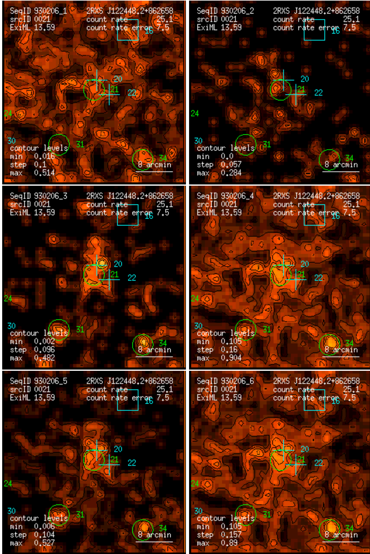
Figure 21: RASS 930206: detection 0021: band rate images, Gaussian filter: (1) PSPC channels 11 – 41, (2) 52 – 90, (3) 91 – 201, (4) 11 – 235, (5) 52 – 201, (6) 11 – 201. Broad band rates in counts/ks. Band rate contour levels in counts/ks/arcmin 2 .
