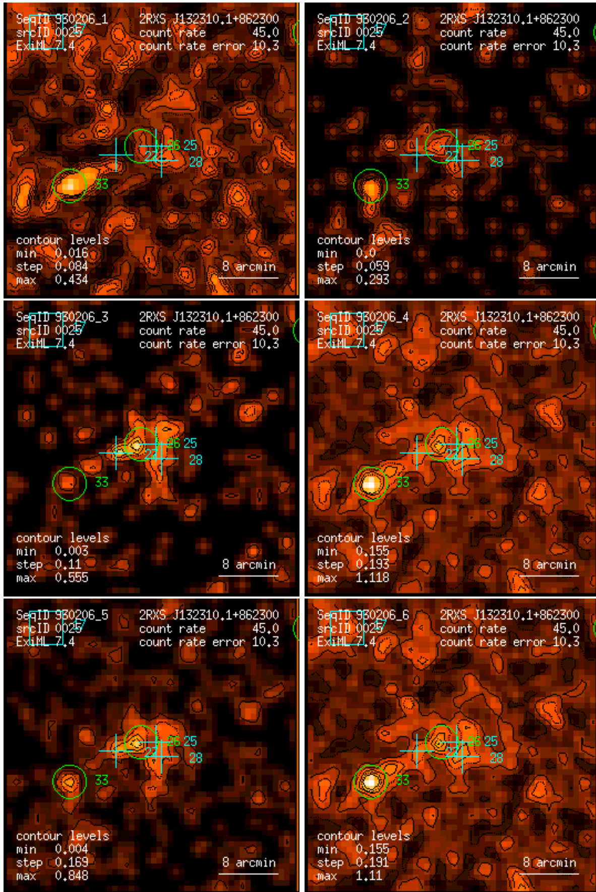
Figure 25: RASS 930206: detection 0025: band rate images, Gaussian filter: (1) PSPC channels 11 – 41, (2) 52 – 90, (3) 91 – 201, (4) 11 – 235, (5) 52 – 201, (6) 11 – 201. Broad band rates in counts/ks. Band rate contour levels in counts/ks/arcmin 2 .
