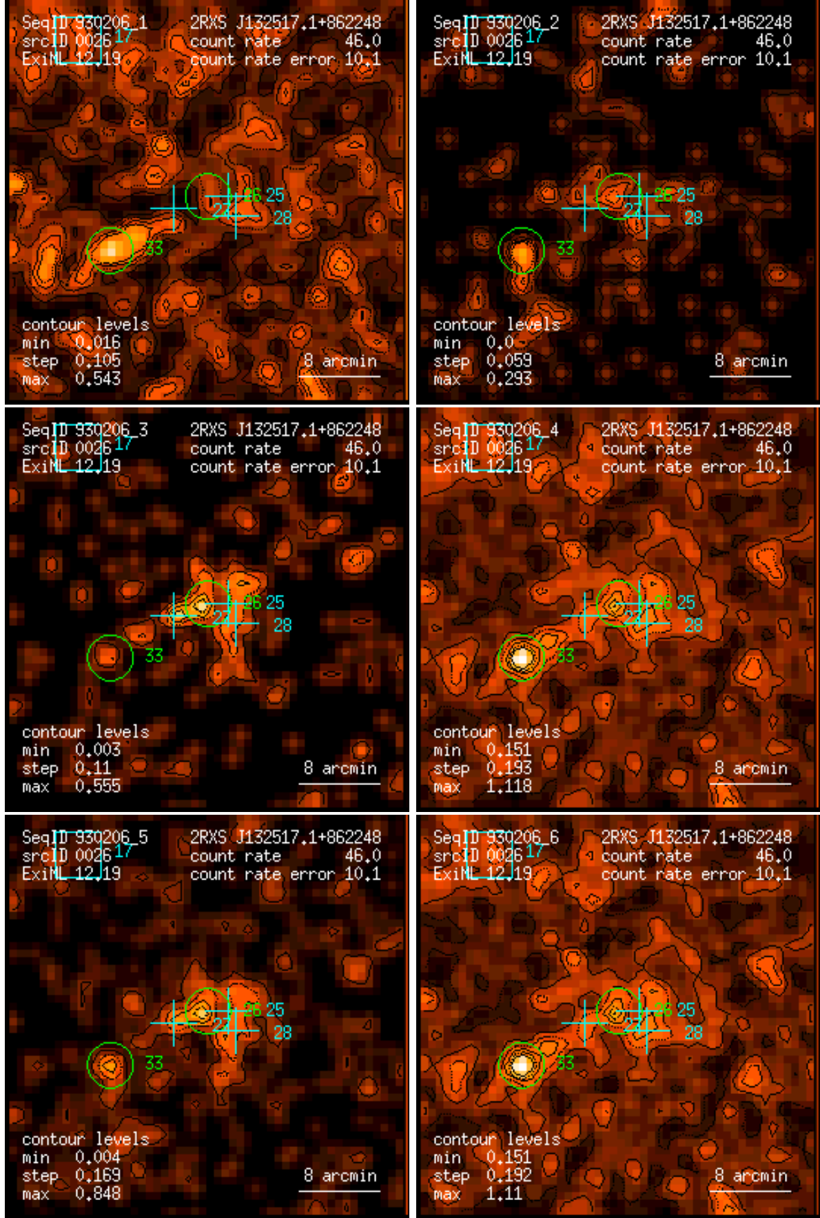
Figure 26: RASS 930206: detection 0026: band rate images, Gaussian filter: (1) PSPC channels 11 – 41, (2) 52 – 90, (3) 91 – 201, (4) 11 – 235, (5) 52 – 201, (6) 11 – 201. Broad band rates in counts/ks. Band rate contour levels in counts/ks/arcmin 2 .
