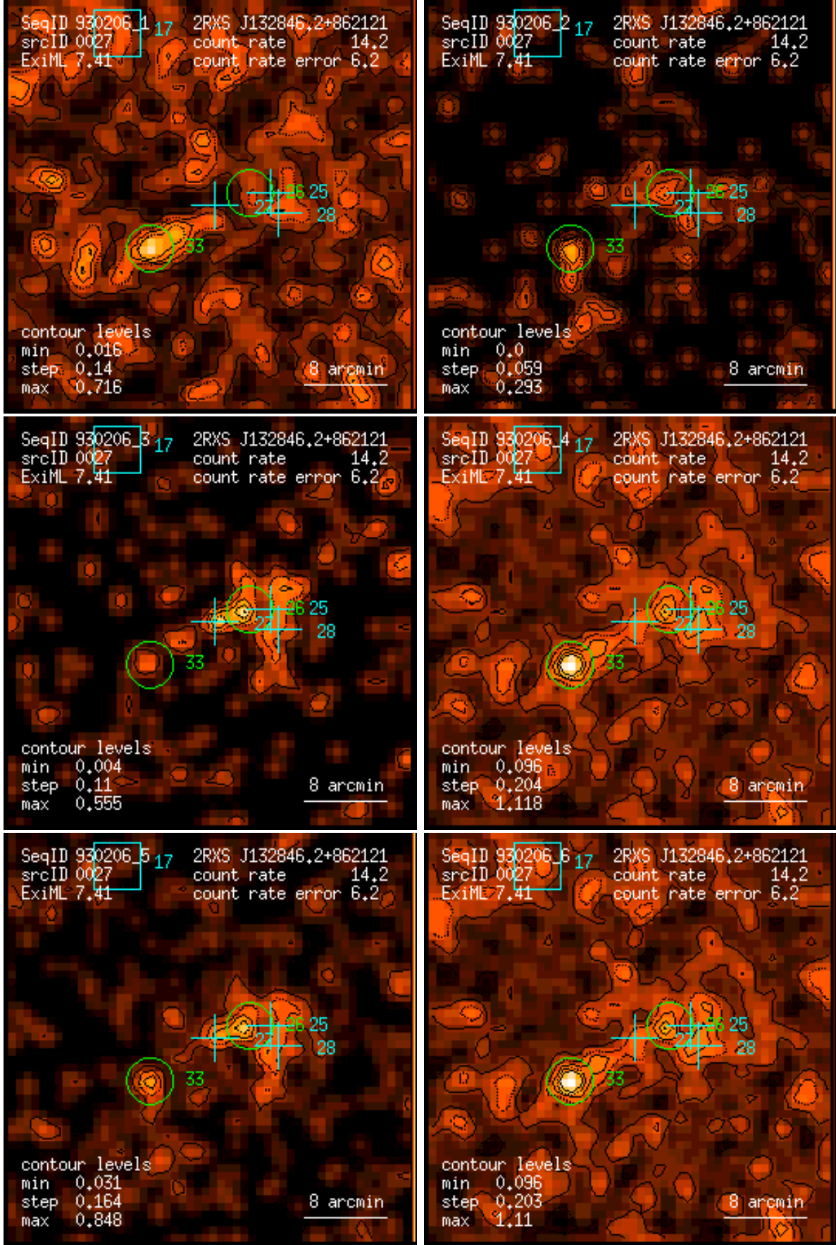
Figure 27: RASS 930206: detection 0027: band rate images, Gaussian filter: (1) PSPC channels 11 – 41, (2) 52 – 90, (3) 91 – 201, (4) 11 – 235, (5) 52 – 201, (6) 11 – 201. Broad band rates in counts/ks. Band rate contour levels in counts/ks/arcmin 2 .
