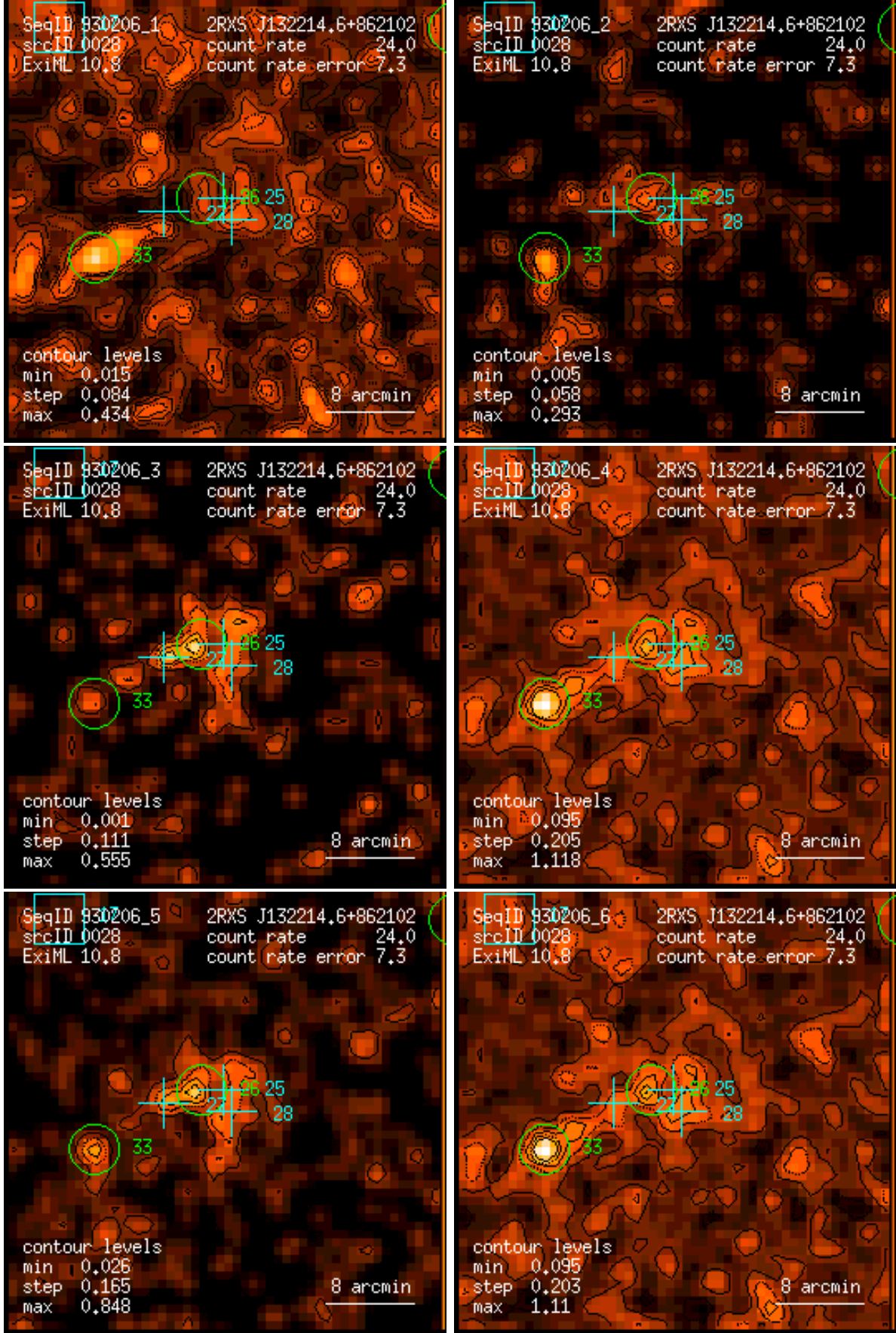
Figure 28: RASS 930206: detection 0028: band rate images, Gaussian filter: (1) PSPC channels 11 – 41, (2) 52 – 90, (3) 91 – 201, (4) 11 – 235, (5) 52 – 201, (6) 11 – 201. Broad band rates in counts/ks. Band rate contour levels in counts/ks/arcmin 2 .
