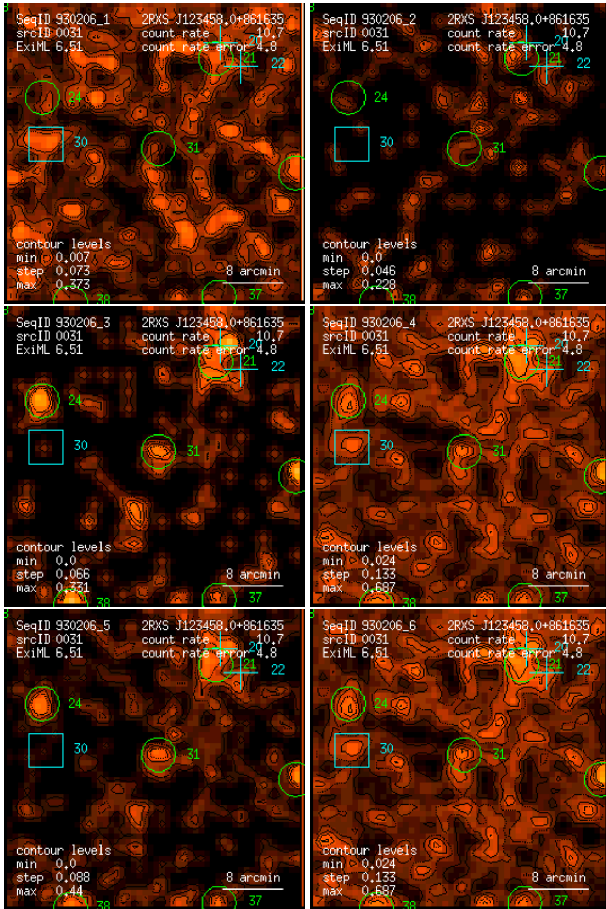
Figure 31: RASS 930206: detection 0031: band rate images, Gaussian filter: (1) PSPC channels 11 – 41, (2) 52 – 90, (3) 91 – 201, (4) 11 – 235, (5) 52 – 201, (6) 11 – 201. Broad band rates in counts/ks. Band rate contour levels in counts/ks/arcmin 2 .
