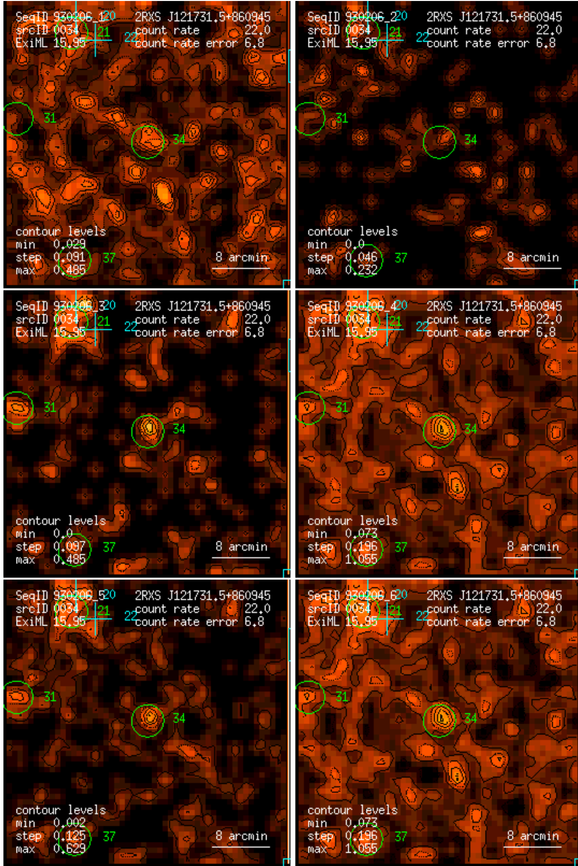
Figure 34: RASS 930206: detection 0034: band rate images, Gaussian filter: (1) PSPC channels 11 – 41, (2) 52 – 90, (3) 91 – 201, (4) 11 – 235, (5) 52 – 201, (6) 11 – 201. Broad band rates in counts/ks. Band rate contour levels in counts/ks/arcmin 2 .
