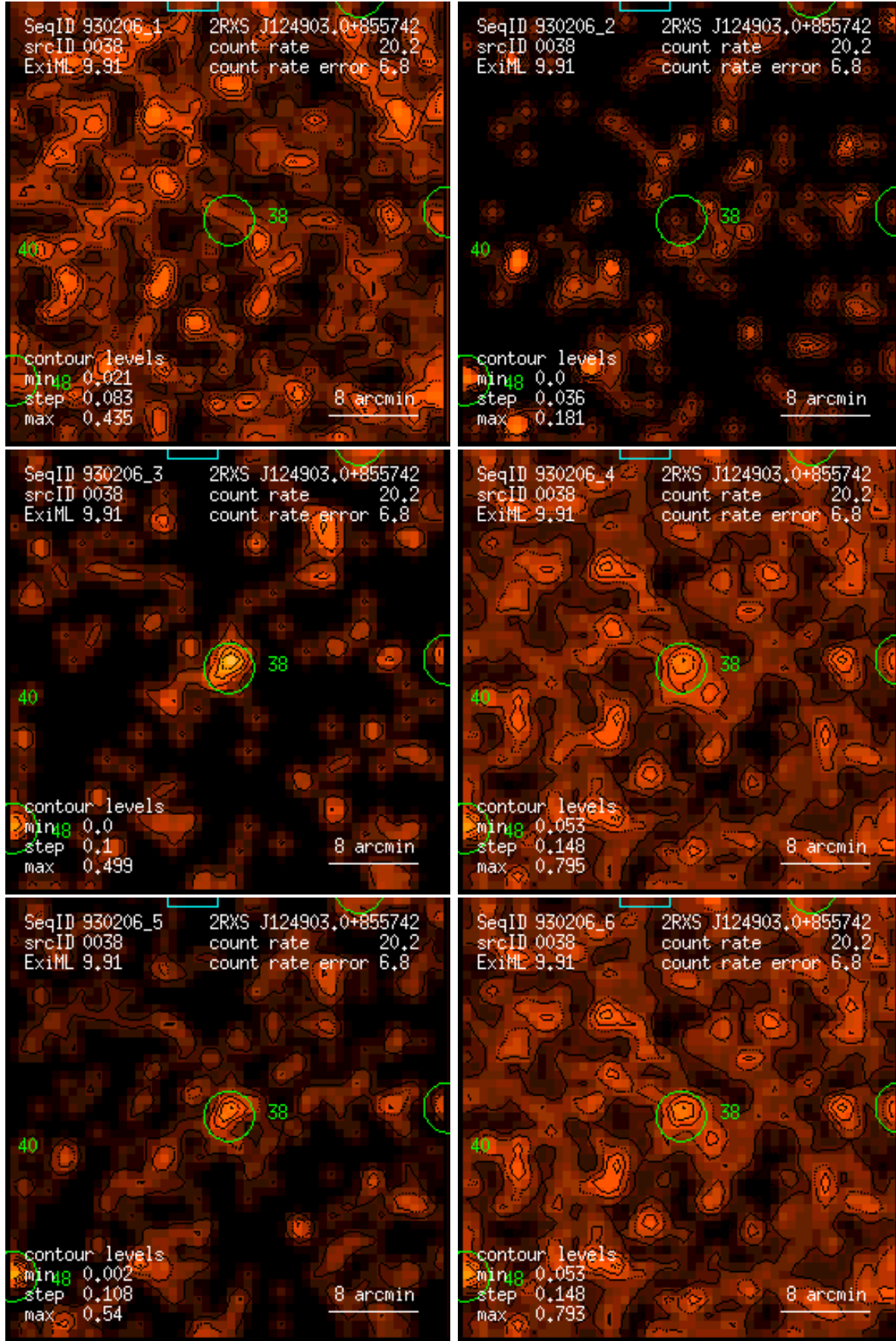
Figure 38: RASS 930206: detection 0038: band rate images, Gaussian filter: (1) PSPC channels 11 – 41, (2) 52 – 90, (3) 91 – 201, (4) 11 – 235, (5) 52 – 201, (6) 11 – 201. Broad band rates in counts/ks. Band rate contour levels in counts/ks/arcmin 2 .
