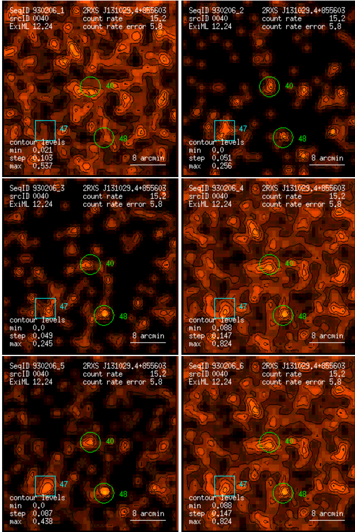
Figure 40: RASS 930206: detection 0040: band rate images, Gaussian filter: (1) PSPC channels 11 – 41, (2) 52 – 90, (3) 91 – 201, (4) 11 – 235, (5) 52 – 201, (6) 11 – 201. Broad band rates in counts/ks. Band rate contour levels in counts/ks/arcmin 2 .
