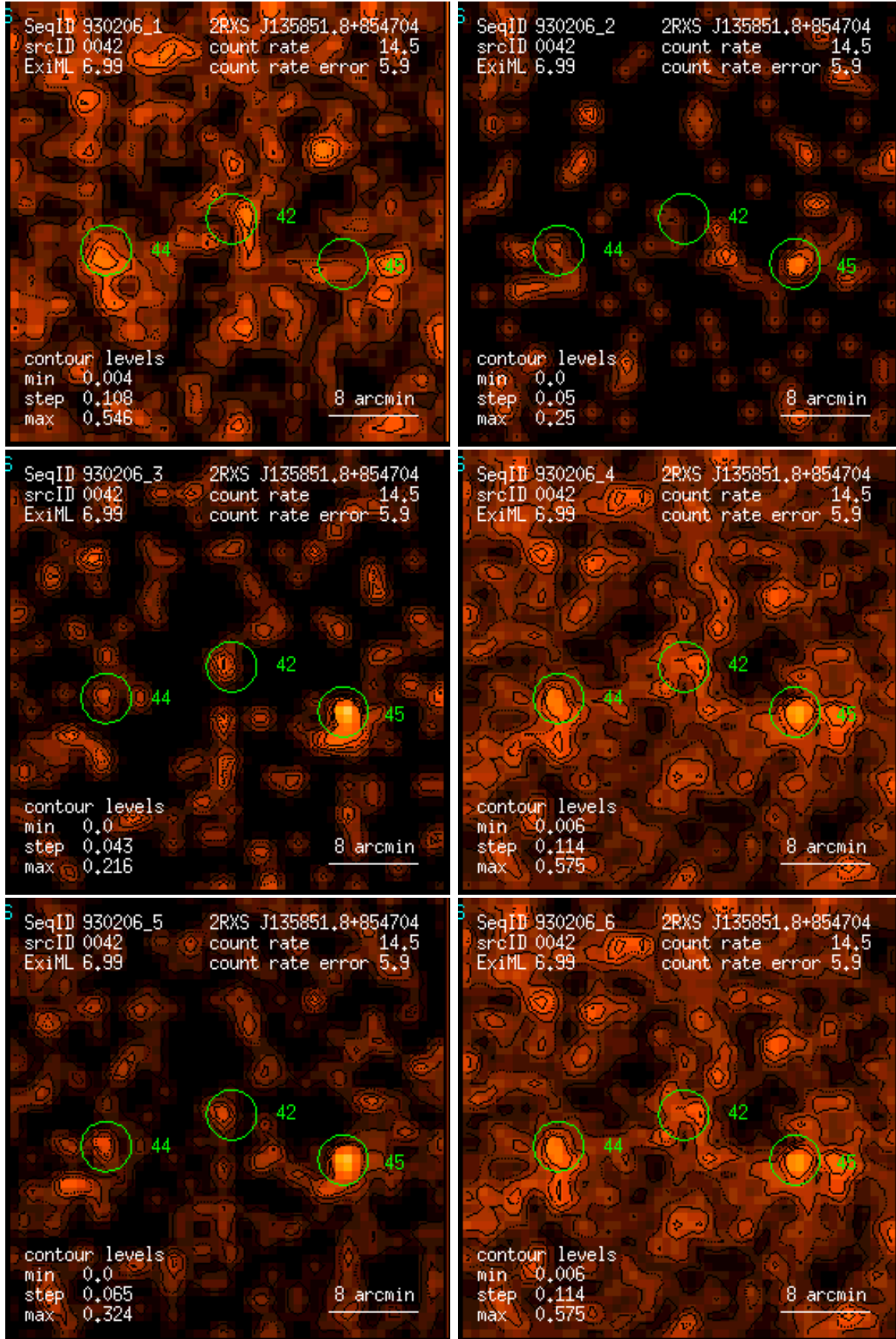
Figure 42: RASS 930206: detection 0042: band rate images, Gaussian filter: (1) PSPC channels 11 – 41, (2) 52 – 90, (3) 91 – 201, (4) 11 – 235, (5) 52 – 201, (6) 11 – 201. Broad band rates in counts/ks. Band rate contour levels in counts/ks/arcmin 2 .
