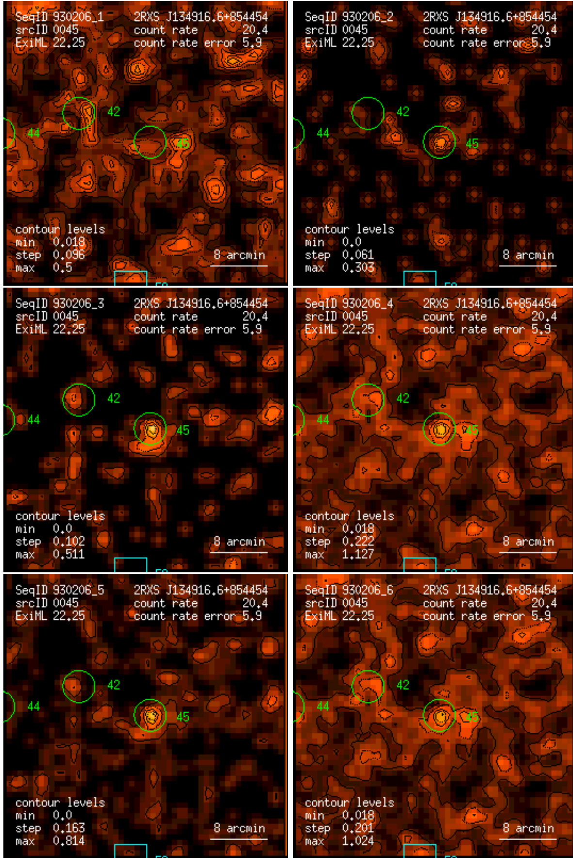
Figure 45: RASS 930206: detection 0045: band rate images, Gaussian filter: (1) PSPC channels 11 – 41, (2) 52 – 90, (3) 91 – 201, (4) 11 – 235, (5) 52 – 201, (6) 11 – 201. Broad band rates in counts/ks. Band rate contour levels in counts/ks/arcmin 2 .
