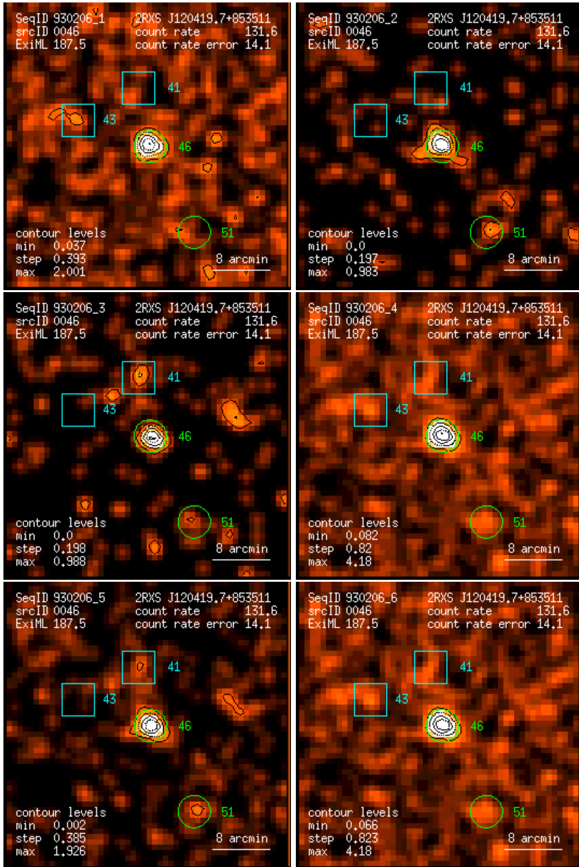
Figure 46: RASS 930206: detection 0046: band rate images, Gaussian filter: (1) PSPC channels 11 – 41, (2) 52 – 90, (3) 91 – 201, (4) 11 – 235, (5) 52 – 201, (6) 11 – 201. Broad band rates in counts/ks. Band rate contour levels in counts/ks/arcmin 2 .
