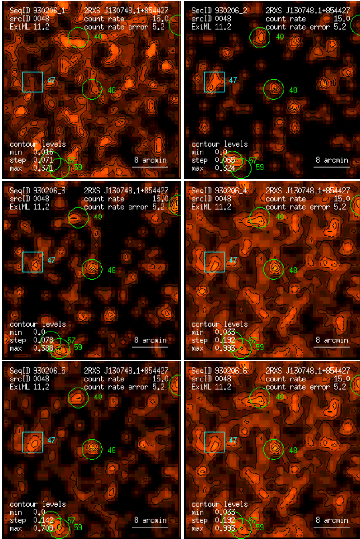
Figure 48: RASS 930206: detection 0048: band rate images, Gaussian filter: (1) PSPC channels 11 – 41, (2) 52 – 90, (3) 91 – 201, (4) 11 – 235, (5) 52 – 201, (6) 11 – 201. Broad band rates in counts/ks. Band rate contour levels in counts/ks/arcmin 2 .
