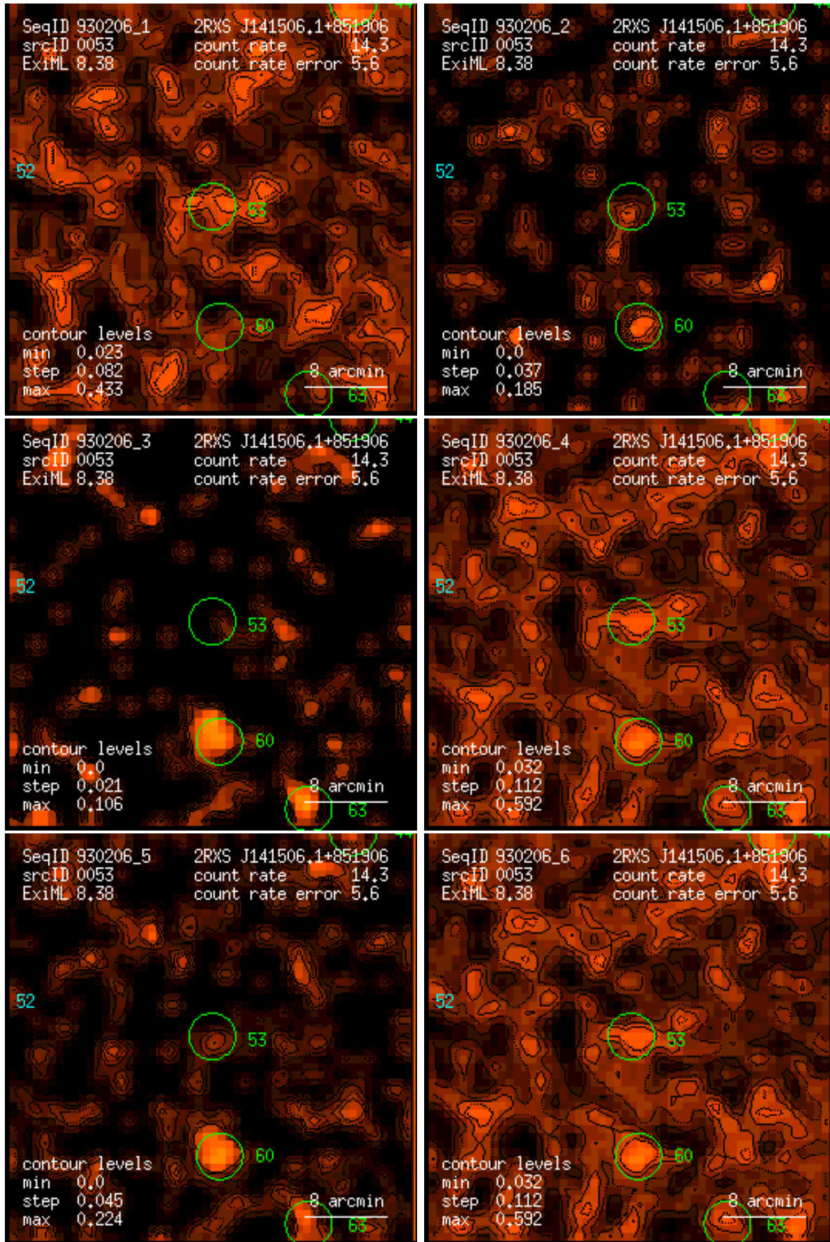
Figure 53: RASS 930206: detection 0053: band rate images, Gaussian filter: (1) PSPC channels 11 – 41, (2) 52 – 90, (3) 91 – 201, (4) 11 – 235, (5) 52 – 201, (6) 11 – 201. Broad band rates in counts/ks. Band rate contour levels in counts/ks/arcmin 2 .
