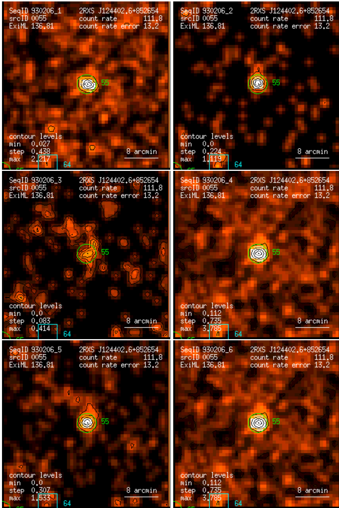
Figure 55: RASS 930206: detection 0055: band rate images, Gaussian filter: (1) PSPC channels 11 – 41, (2) 52 – 90, (3) 91 – 201, (4) 11 – 235, (5) 52 – 201, (6) 11 – 201. Broad band rates in counts/ks. Band rate contour levels in counts/ks/arcmin 2 .
