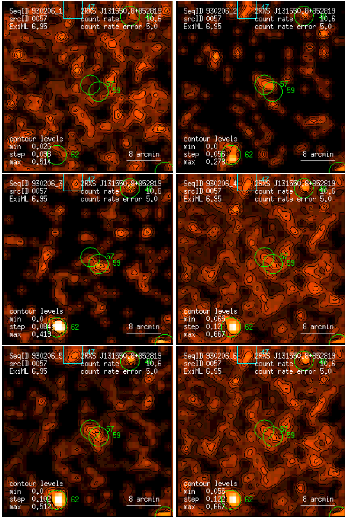
Figure 57: RASS 930206: detection 0057: band rate images, Gaussian filter: (1) PSPC channels 11 – 41, (2) 52 – 90, (3) 91 – 201, (4) 11 – 235, (5) 52 – 201, (6) 11 – 201. Broad band rates in counts/ks. Band rate contour levels in counts/ks/arcmin 2 .
