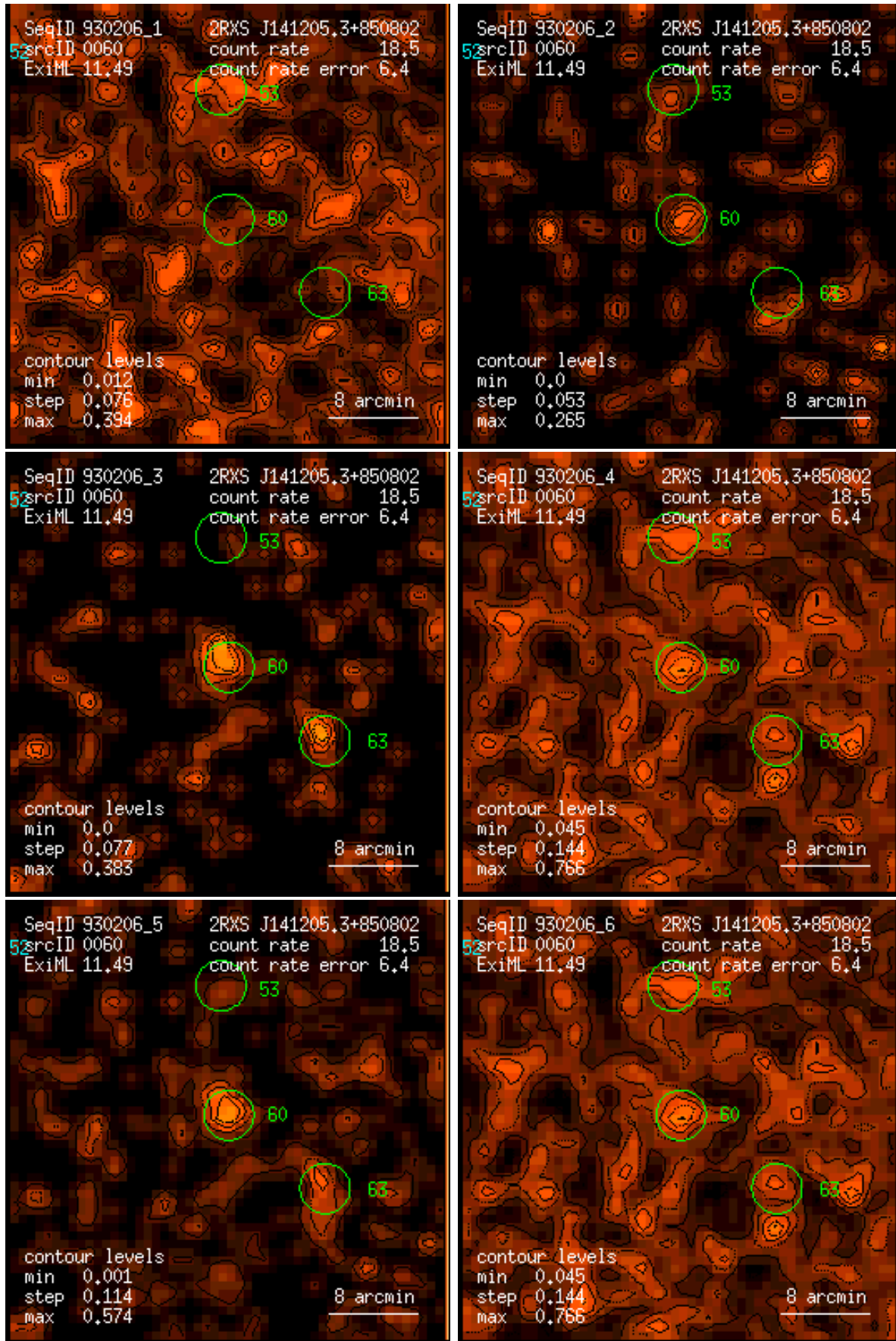
Figure 60: RASS 930206: detection 0060: band rate images, Gaussian filter: (1) PSPC channels 11 – 41, (2) 52 – 90, (3) 91 – 201, (4) 11 – 235, (5) 52 – 201, (6) 11 – 201. Broad band rates in counts/ks. Band rate contour levels in counts/ks/arcmin 2 .
