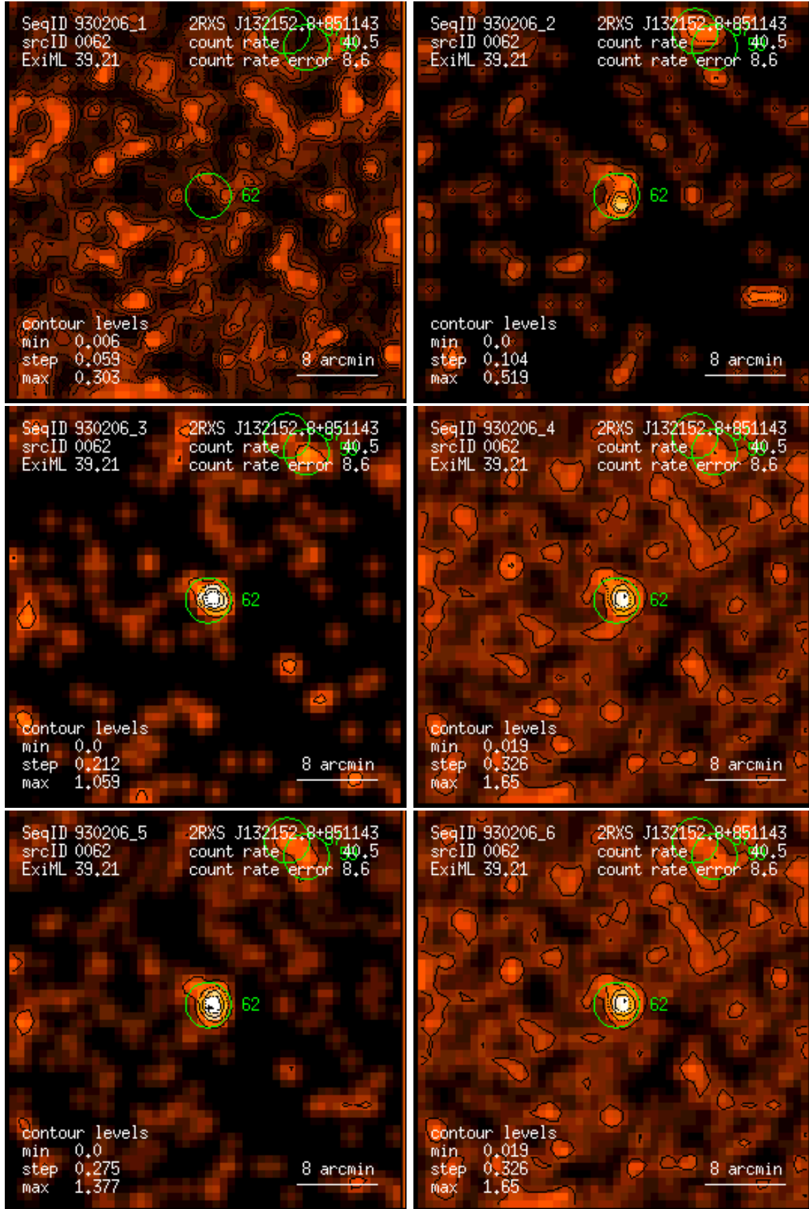
Figure 62: RASS 930206: detection 0062: band rate images, Gaussian filter: (1) PSPC channels 11 – 41, (2) 52 – 90, (3) 91 – 201, (4) 11 – 235, (5) 52 – 201, (6) 11 – 201. Broad band rates in counts/ks. Band rate contour levels in counts/ks/arcmin 2 .
